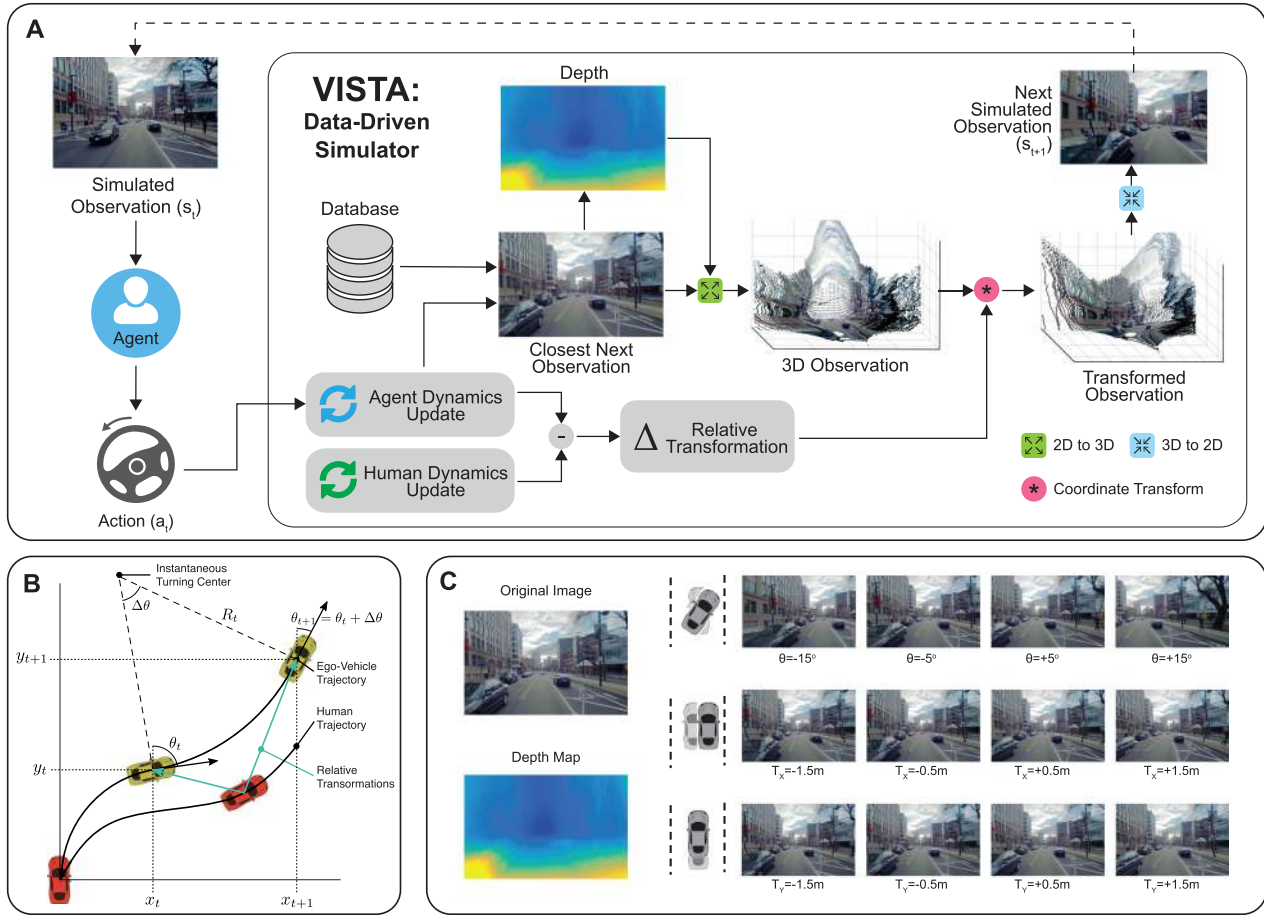
Fig. 2. Simulating novel viewpoints for learning: Schematic of an autonomous agent's interaction with the data-driven simulator (A). At time step, t , the agent receives an observation of the environment and commands an action to execute. Motion is simulated in VISTA and compared to the human's estimated motion in the real world (B). A new observation is then simulated by transforming a 3D representation of the scene into the virtual agent's viewpoint (C).
