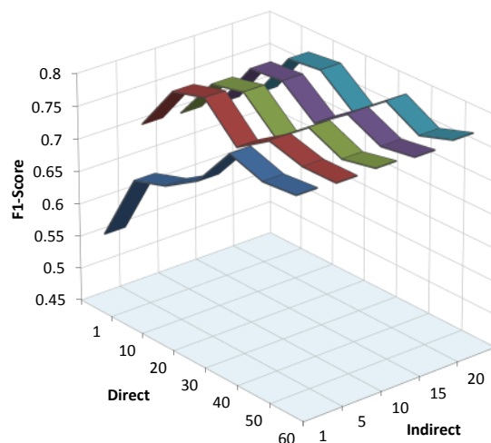
Figure 6: Performance on development data w.r.t. cluster size.
