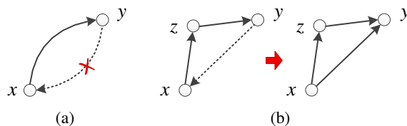
Figure 5: (a) If d(\Phi_j y, x) > d(\Phi_k x, y) , we remove the path from y to x ; (b) if d(\Phi_k x, z) > d(\Phi_j y, x) and d(\Phi_j y, x) > d(\Phi_i z, y) , we reverse the path from y to x .
