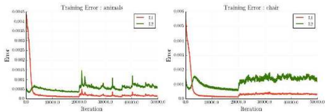
Figure 5: We plot the Coverage (L1) and Consistency (L2) losses over training iterations. The losses both decrease in the initial stage of training (up to 20,000 iterations) but when we allow the use of varying number of primitives along with parsimony reward, the losses initially increase. This reveals a tradeoff between representation parsimony and reconstruction accuracy.
