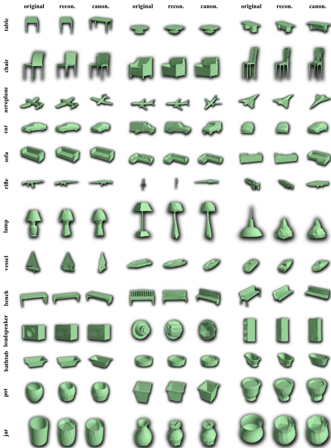
Fig. 6 Qualitative examples of reconstructions for different object classes. Each group of three images shows (i) ShapeNet ground-truth; (ii) our reconstruction; (iii) reconstruction placed in a canonical pose,
