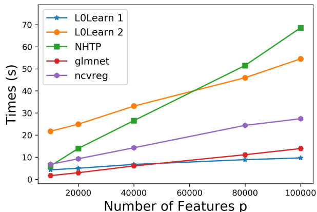
Figure 4: Running time to obtain good feasible solutions: Time (s) for obtaining a regularization path (with 100 solutions) for different values of p (as discussed in Section 5.5.1). L0Learn 1 runs Algorithm 1 (CD), while L0Learn 2 runs Algorithm 2 (CD with Local Search).
