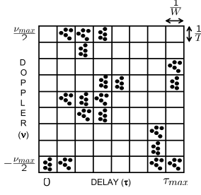
Fig. 1. A schematic illustrating the virtual representation of a single-antenna, doubly-selective channel. Each black dot denotes the contribution of a distinct physical path to the delay-Doppler spreading function and the virtual channel coefficients \{h_{\ell,k}\} correspond to uniformly-spaced samples of a smoothed version of the spreading function taken at \{(\tau_\ell, \nu_k) = (\ell/W, k/T)\} .
