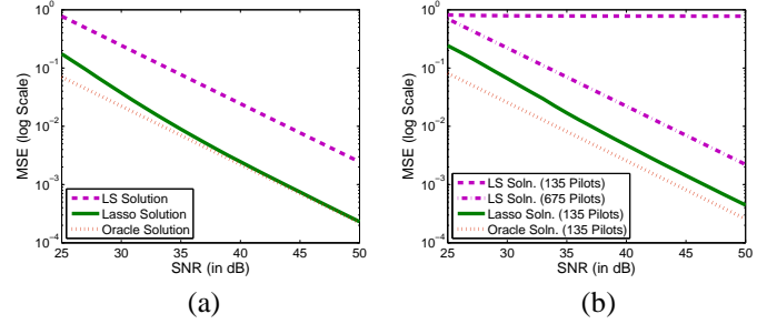
Fig. 2. Numerical results comparing the performance of a lasso estimator with that of a LS estimator. The MSEs of the channel estimates are plotted on a log scale against the SNR in dB corresponding to (a) Spread Spectrum Training Waveforms, and (b) STF Training Waveforms.
