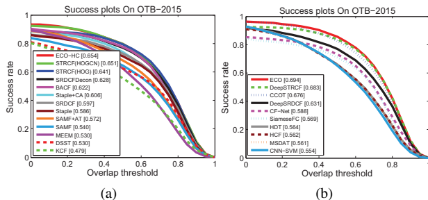
Figure 3: A comparison of the overlap success plots with the state-of-the-art trackers on OTB-2015 dataset. (a) Trackers with hand-crafted features. (b) Trackers with deep features.
