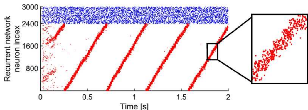
Fig 2. Learning a sequential dynamics stably under plasticity. (A) The excitatory neurons receive sequential clustered inputs. Excitatory neurons are grouped in 30 disjoint clusters of 80 neurons each. (7 clusters shown in the cartoon for simplicity) (B) The weight matrix after training (only the first five clusters shown) exhibits the learned connectivity structure, e.g., neurons within cluster 1 are highly interconnected and also project to neurons in cluster 2, same for cluster 2 to cluster 3, etc. The spectrum of the full weight matrix after training shows most eigenvalues in a circle in the complex plane (as in a random graph) with two other eigenvalues signifying the balancing of the network, and a
