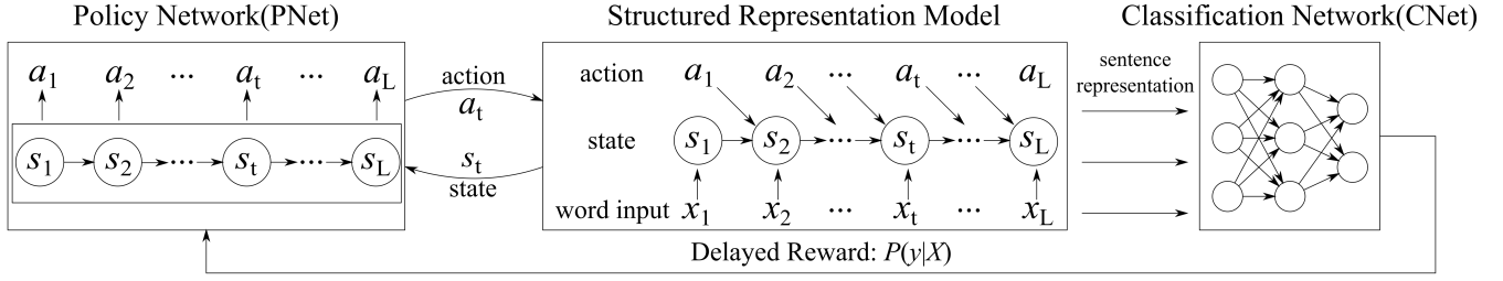
Figure 1: Illustration of the overall process. The policy network (PNet) samples an action at each state. The structured representation model offers state representation to PNet and outputs the final sentence representation to the classification network (CNet) when all actions are sampled. CNet performs text classification and provides reward to PNet.
