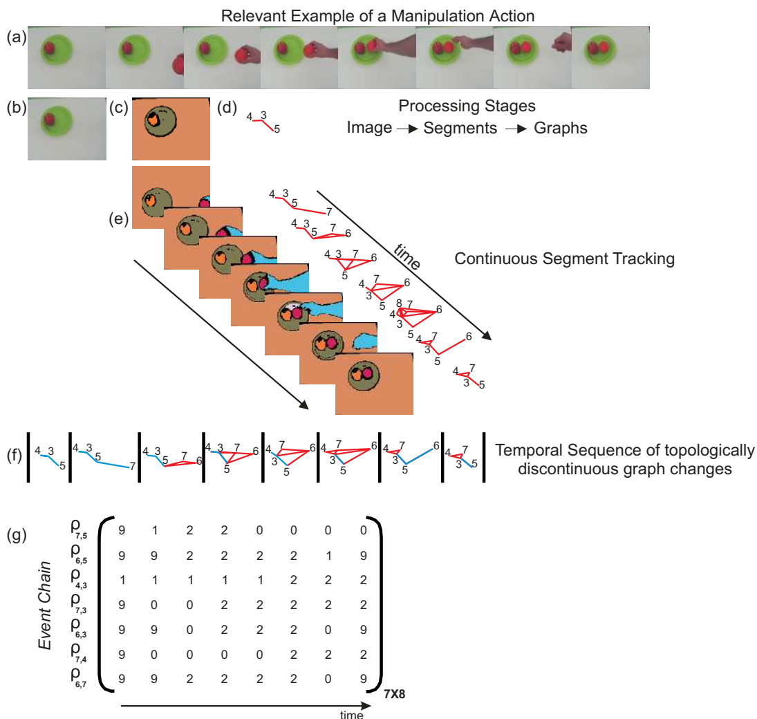
Figure 1: Processing example and semantic event chain representation. (a) Frames from a movie recorded during a manipulation. All frames (b) are segmented (c) by superparamagnetic clustering in a spin-lattice model (Dellen et al., 2009), which also allows for consistent marker-less tracking (e) of the individual segments. From the image segments, graphs are constructed (d) where graph nodes represent the segments' centers and graph edges encode whether or not two segments touch each other. Then we encode a manipulation by storing only main graphs between which a topological change has taken place (f). Such a change happens whenever an edge or a node has been newly formed or has been deleted. This type of representation is then given by the semantic event chain (g), which is a sequence-table, where each entry encodes the spatial relations between each segment pair \rho_{i,j} counting graph edges (2 means that segments touch (denoted by red edges), 1 means that they overlap (denoted by blue edges), 0 means that there is no edge between two segments, and absence of a previously existing segment yields 9).
