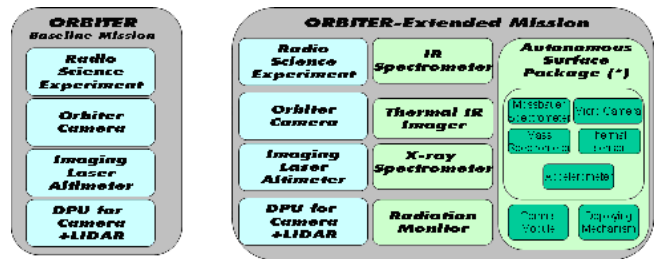
Figure 5: Orbiter’s payload
