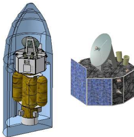
Figure 6: Hidalgo's launch and flight configuration
