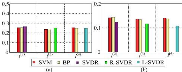
Figure 7. Results on DS2.
