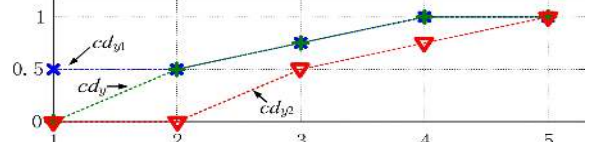
Figure 5. The cumulative distribution functions of y , y_1 and y_2 .
