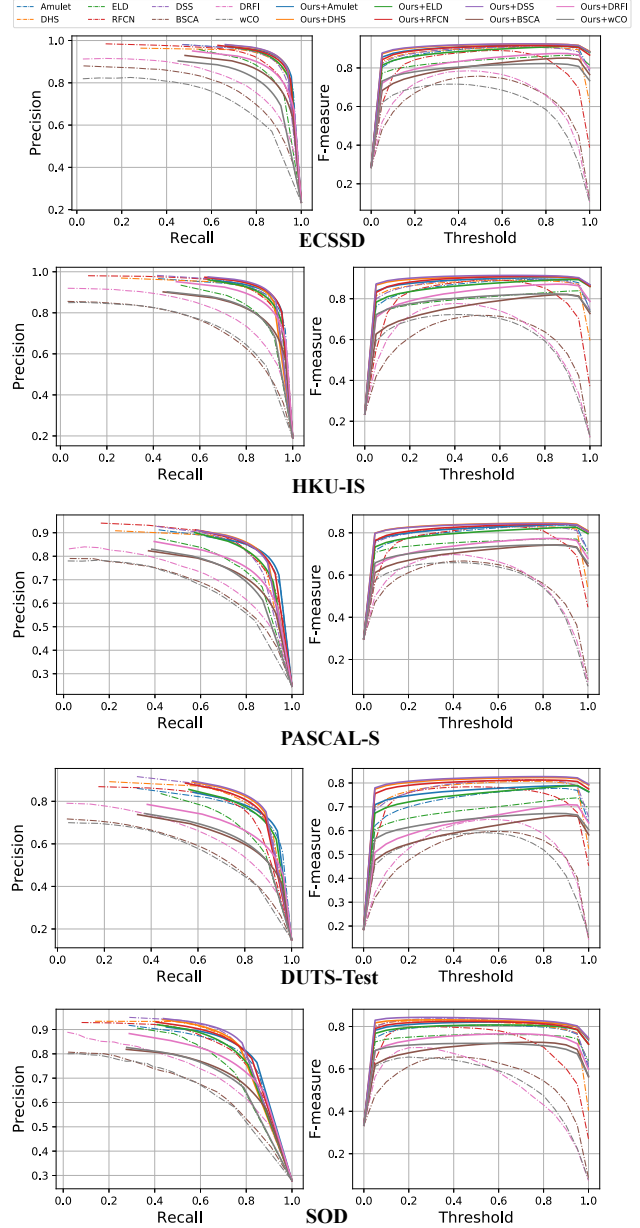
Figure 6. PR curves and F-measure curves of our method and the the state-of-the-art methods.
