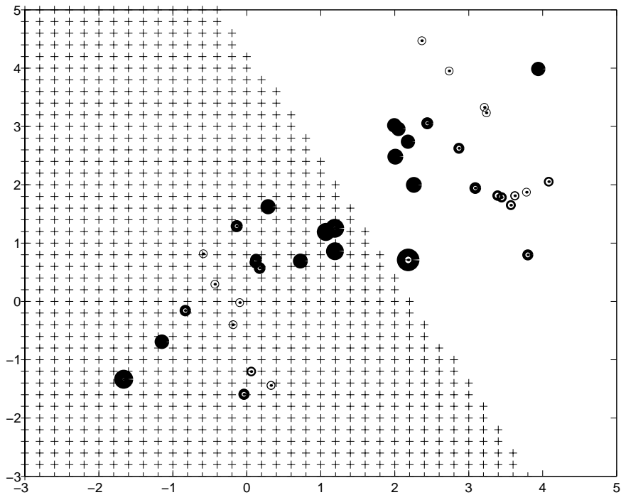
Figure 1. Example of two linearly separable classes in a two-dimensional input space. The size of the circles indicated at the training data is chosen proportionally to the absolute value of the support value.
