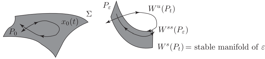
FIGURE 6.2. (a) Phase portrait on \Sigma for \epsilon = 0 . (b) Perturbation of invariant manifolds, \epsilon > 0 .
