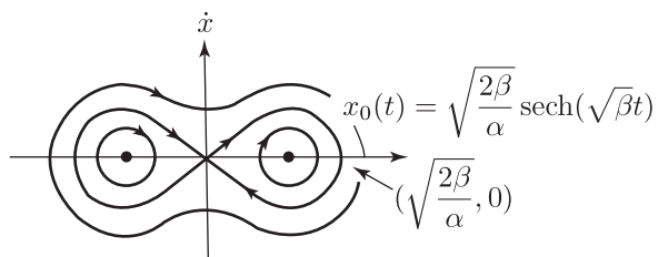
FIGURE 6.4. The homoclinic orbit in Duffing's equation.
