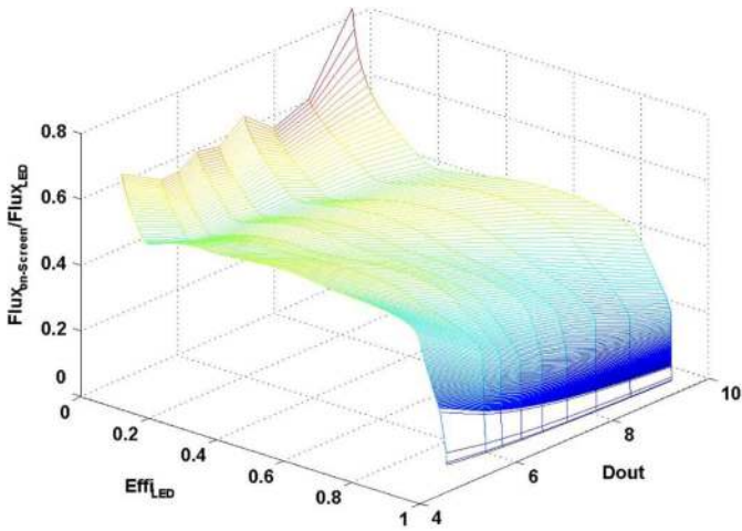
Fig. 7. ((\eta_{I,LED}) / (\Omega_{I,LED} A_{pack})) \Omega_{I,A}, \eta_{I,E} versus \eta_{I,LED} parameter space for the CPC array.
