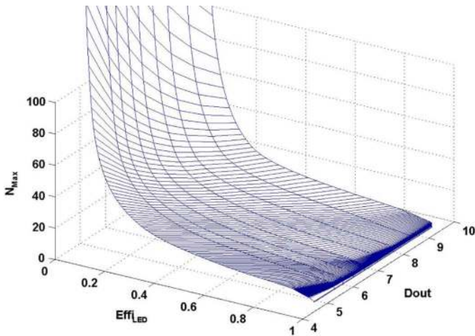
Fig. 8. Maximum LED number N versus \eta_{I,LED} parameter space for the CPC array.
