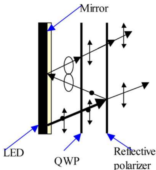
Fig. 10. Structure of the polarization converter and its polarization conversion efficiency.
