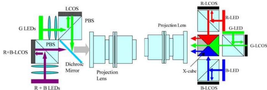
Fig. 14. Two-/three-panel system configurations.
