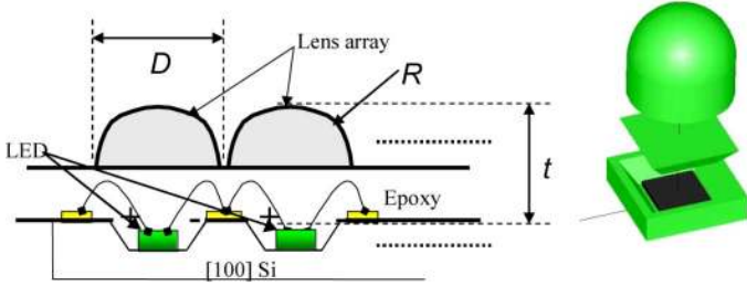
Fig. 3. Structure of LED lens array.
