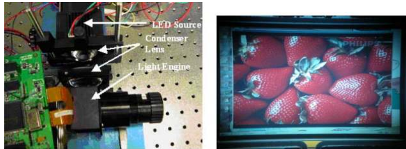
Fig. 12. Practical blue-LED + yellow-phosphor-based one-panel system and its projected image.
