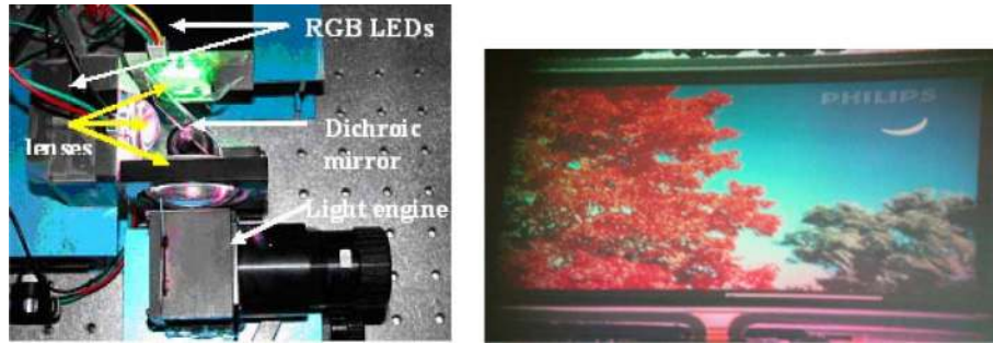
Fig. 13. Practical RGB-LED-based one-panel system and its projected image.
