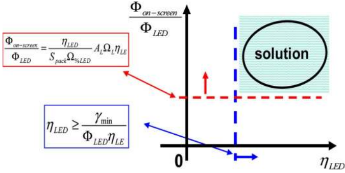
Fig. 2. Parameter space with minimum requirements or boundaries.
