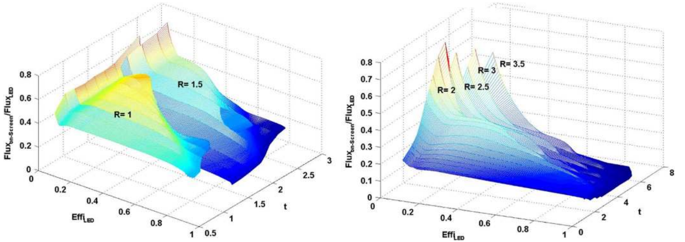
Fig. 4. ((\eta_{LED})/(\Omega_{LED} A_{pack}))\Omega_{t,A,t,\eta_{LED}} versus \eta_{LED} parameter space for the lens array.
