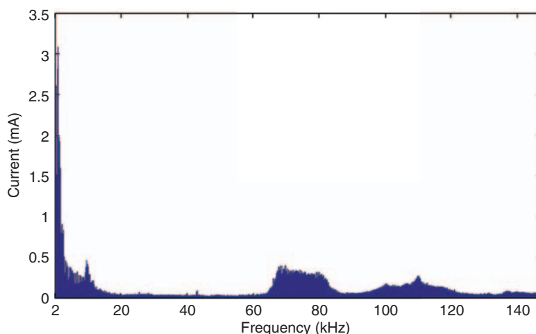
Figure 9 The 200-Hz band spectrum of the current feeding the HPS lamp connected to electronic ballast in the range from 2 to 150 kHz
