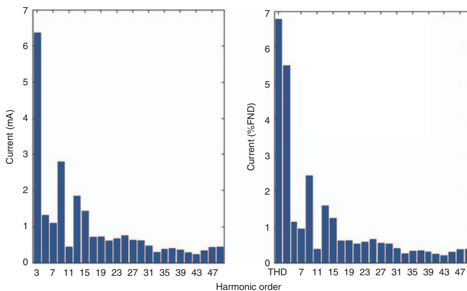
Figure 2 Harmonic current spectrum from a LED street light lamp in milliamperes and percentage of fundamental
