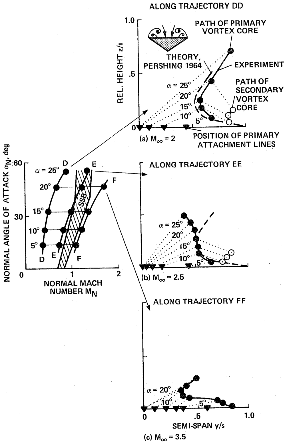
Figure 6.- Vortex center and primary attachment line position for thick wings (Szodruich, 1977).
