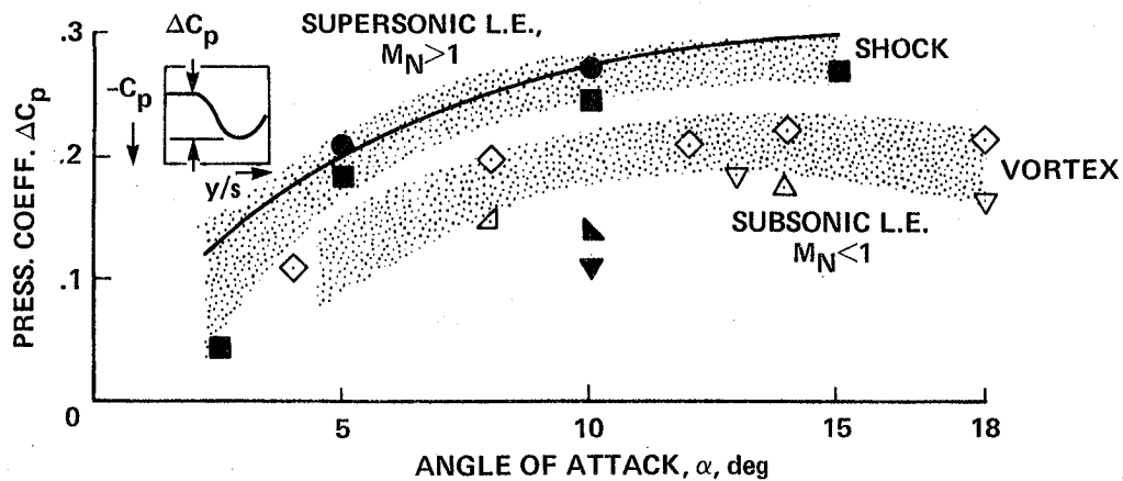
(b) DIFFERENCE BETWEEN PRESSURES AT PRIMARY ATTACHMENT LINE AND PRIMARY VORTEX CENTER LOCATION PROJECTED ON WING
