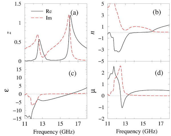
FIG. 3. (Color online) Effective material parameters, impedance ( z ), refractive index ( n ), permittivity ( \epsilon ), and permeability ( \mu ) for the fishnet structure of Fig. 2(b). The solid lines show the real part of the parameters, the dashed lines the imaginary part, and the dotted horizontal lines are guides for the eyes.
