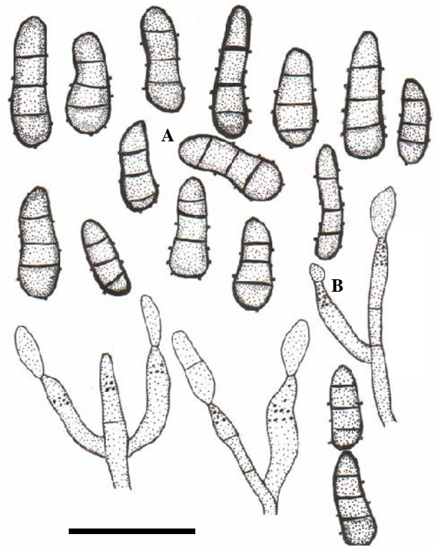
Figure 12. Fusariella aegyptiaca (A) Conidia, (B) Phialides. Bar = 25 \mu m
