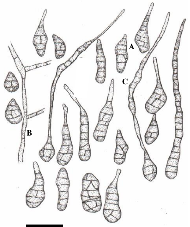
Figure 2. Alternaria dianthi (A) Conidia, (B) Conidiophores, (C) Chlamydospores. Bar = 50 \mu m
