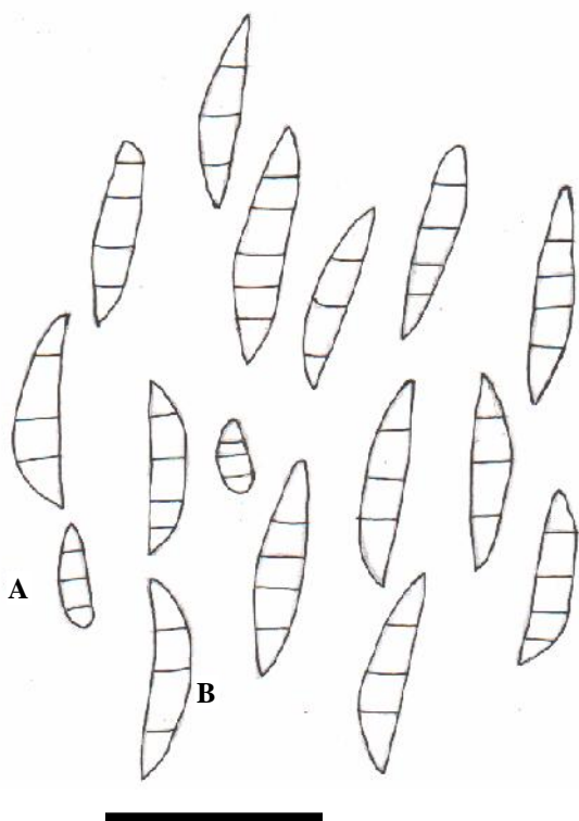
Figure 15. Fusarium semitectum (A) Primary microconidia, (B) Secondary macroconidia. Bar = 25 \mu m
