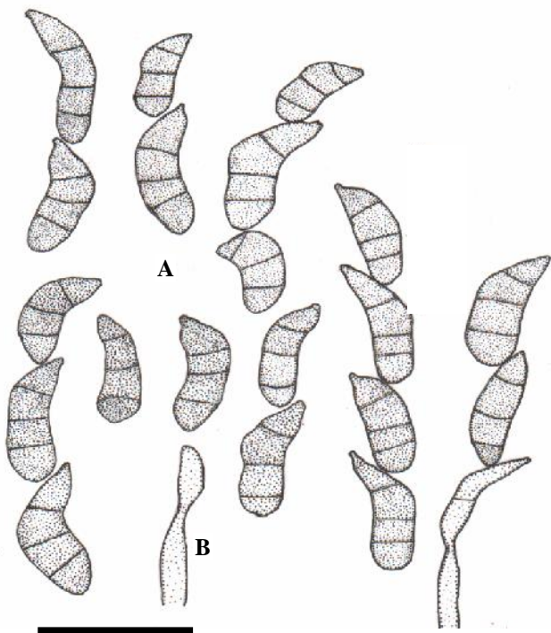
Figure 13. Fusariella intermedia (A) Conidia, (B) Phialides. Bar = 25 \mu m
