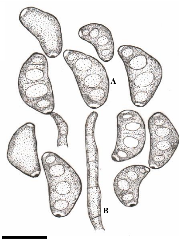
Figure 9. Drechslera papendorfii (A) Conidia, (B) Conidiophores. Bar = 25 \mu m
