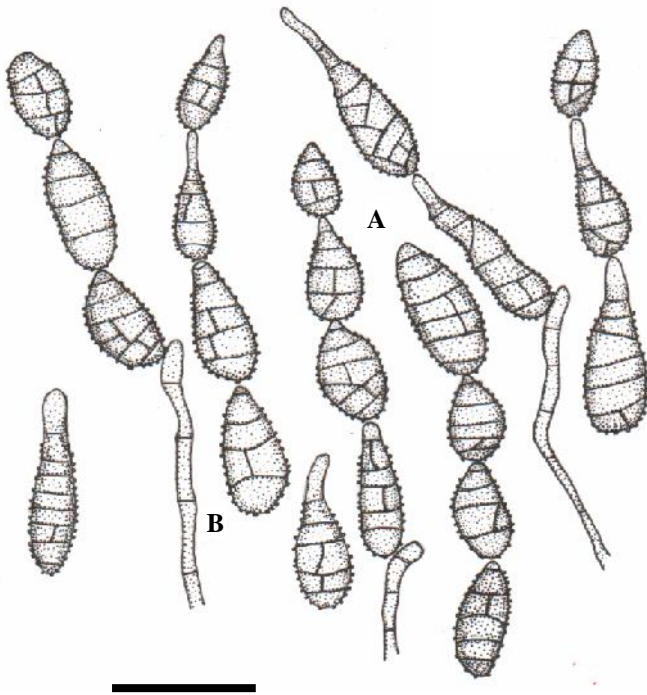
Figure 1. Alternaria alternata (A) Conidia, (B) Conidiophores. Bar = 50 \mu m
