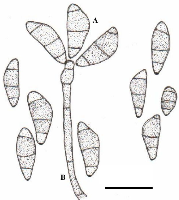
Figure 8. Curvularia pallescens (A) Conidia, (B) Conidiophores. Bar = 25 \mu m
