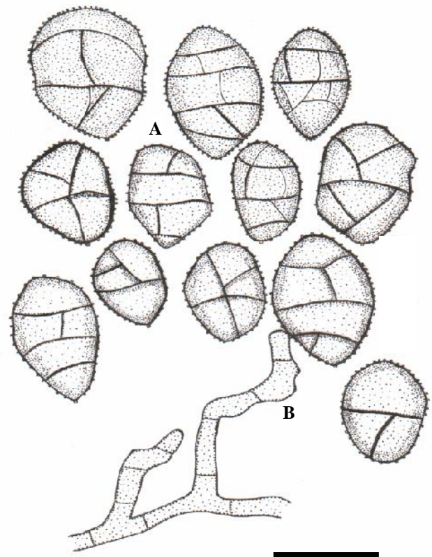
Figure 18. Ulocladium botrytis (A) Conidia, (B) Conidiophores. Bar = 25 \mu m
