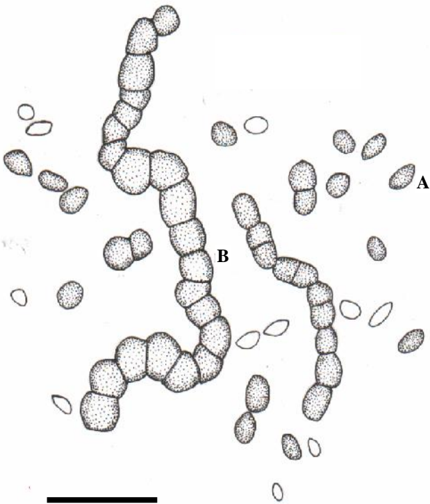
Figure 5. Aureobasidium pullulans (A) Conidia, (B) Conidiophores. Bar = 50 \mu m
