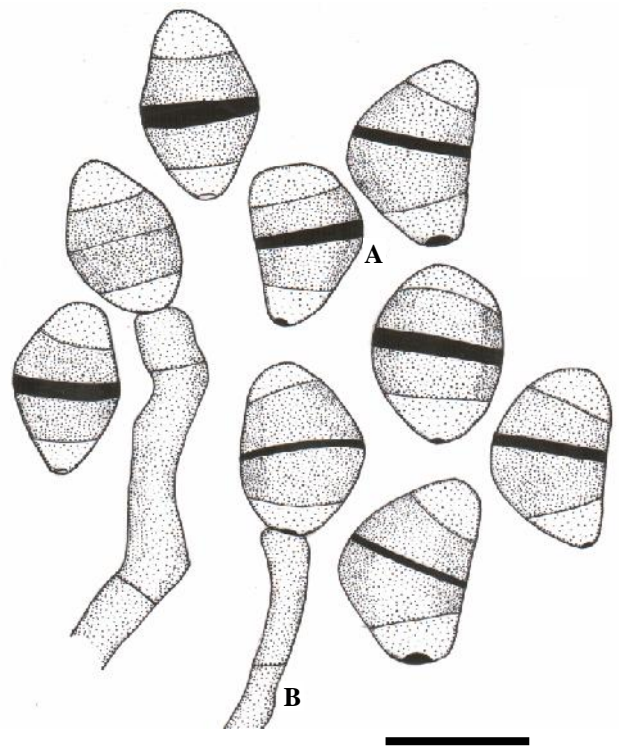
Figure 6. Curvularia brachyspora (A) Conidia, (B) Conidiophores. Bar = 25 \mu m
