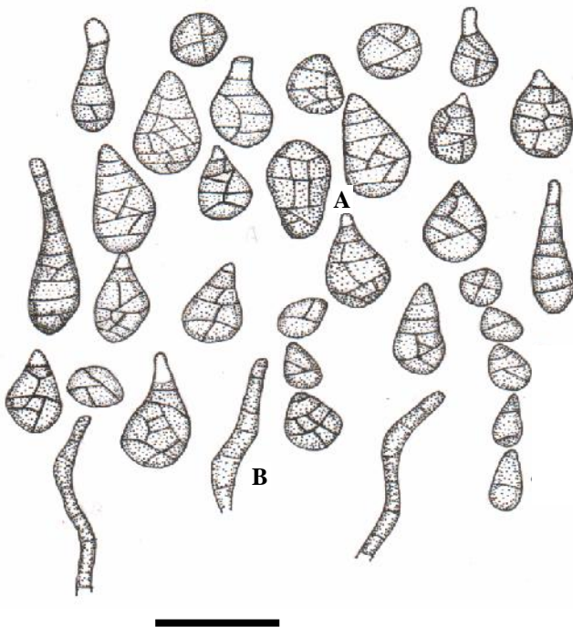
Figure 3. Alternaria tenuis (A) Conidia, (B) Conidiophores. Bar = 50 \mu m
