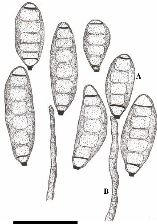
Figure 10. Drechslera rostrata (A) Conidia, (B) Conidiophores. Bar = 50 \mu m
