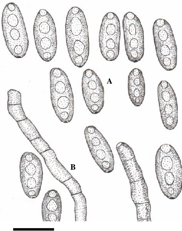
Figure 11. Drechslera spicifera (A) Conidia, (B) Conidiophores. Bar = 50 \mu m
