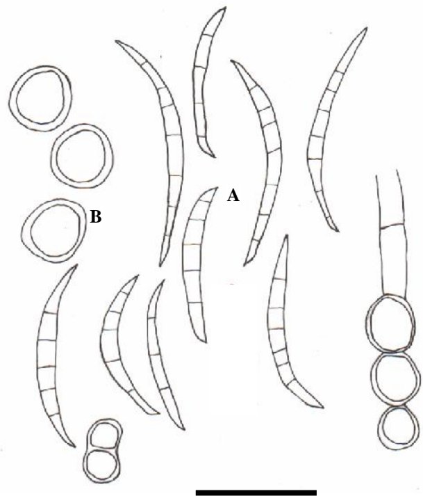
Figure 14. Fusarium equiseti (A) Macroconidia, (B) Chlamydospores. Bar = 25 \mu m
