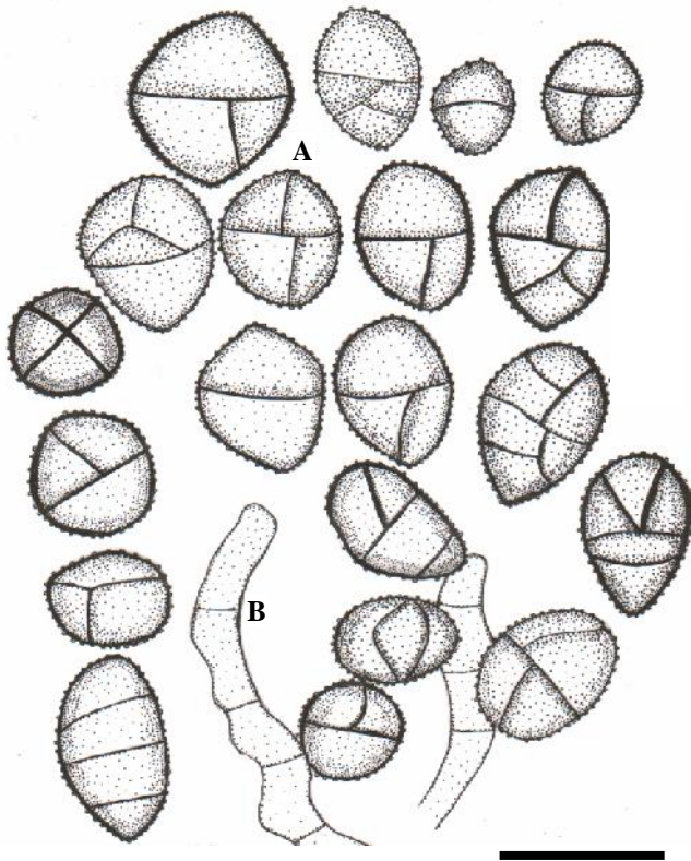
Figure 17. Ulocladium atrum (A) Conidia, (B) Conidiophores. Bar = 25 \mu m
