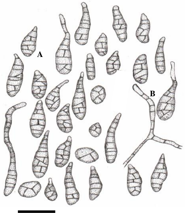
Figure 4. Alternaria tenuissima (A) Conidia, (B) Conidiophores. Bar = 50 \mu m
