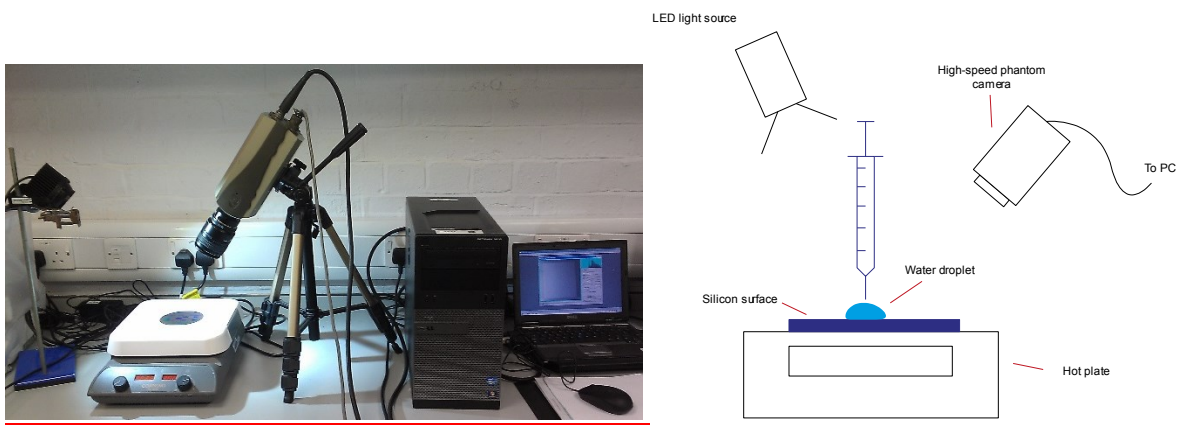
Figure 4 Schematic of apparatus (colour online)
