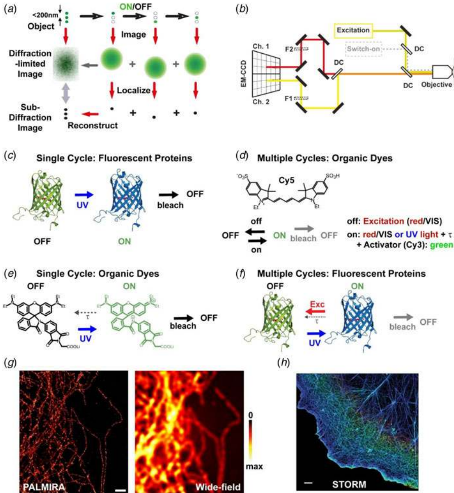
Fig. 12. Coordinate-stochastic (single-marker/single-molecule switching-based) nanoscopy ((F)PALM/STORM). (a) Images with sub-diffraction spatial resolution are reconstructed from consecutive camera frames with simultaneous imaging and position-localization of single isolated (sparse) molecules only, which are switched on and off one after the other. (b) The setup is typically based on a conventional wide-field (TIRF) microscope with an excitation laser and, if required, an additional switching (or activation) laser, a microscope objective, dichroic mirrors (DC) for overlaying the lasers, de-coupling the fluorescence signal from the laser light and if required splitting up the fluorescence signal into two different wavelength ranges, fluorescence filters (here F1 and F2) for rejecting any residual laser scattering light and selecting the detected wavelength range, and a CCD camera detecting the fluorescence potentially in two channels (Ch. 1 and Ch. 2). (c–f) Various modes of (F)PALM/STORM-based nanoscopy differing in the labels and molecular transitions: (c) the original (F)PALM approach using photoactivatable proteins that are initially dark or non-detectable, sparsely switched on by, for example, UV light and switched off by photobleaching. (d) The original STORM approach: Organic dyes such as Cy5 (or also fluorescent proteins) can be switched on and off by laser light of the same or different color or by spontaneous recovery ( \tau ), with on- and off-switching potentially assisted by an additional activator dye such as Cy3 and by photobleaching, respectively. (e) Single-cycle switching using photoactivatable organic dyes that are initially dark or non-detectable, sparsely switched on by UV light and switched off by photobleaching or rarely by a spontaneous dark state return ( \tau ). (f) Multiple-cycle switching using RSFPs that can be switched between a dark and bright isomer using the excitation and UV light (or spontaneous transitions ( \tau ) and photobleaching). (g) Example PALM/STORM image of a tubulin network in a fixed PtK2 cell stained with a photoactivatable rhodamine
