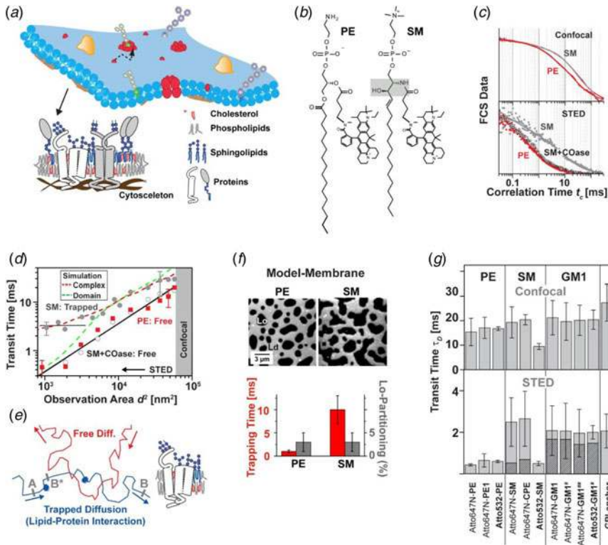
Fig. 9. STED-FCS analysis of lipid plasma membrane diffusion. (a) Lipids and proteins are heterogeneously distributed in the cellular plasma membrane, stemming from often cholesterol-assisted lipid–protein interactions (which may be the basis for the coalescence of transient signaling platforms, denoted membrane domains or lipid ‘rafts’, i.e. spatially confined molecular assemblies of different lipids and proteins which are essential for a cellular signaling event), an asymmetric molecular distribution to the inner and outer leaflet of the bilayer, the underlying cytoskeleton (which is membrane-anchored via proteins), and from membrane curvature and pits. Adapted from (Lingwood & Simons, 2010). (b) Structures of the fluorescent lipid analogs phosphoethanolamine (PE) and sphingomyelin (SM), both tagged with the organic dye Atto647N. Grey shaded area: ceramide or sphingosine group of the SM lipid. (c) Representative confocal and STED (observation diameter d = 40 nm) FCS data of PE (red), SM (black) and SM after cholesterol depletion by Cholesterol Oxidase (grey, SM+COase). The SM STED-FCS data can only be described by anomalous diffusion, revealing cholesterol-assisted hindered diffusion of the SM lipid analog. (d) The dependence of the transit time \tau_D for different sub-diffraction sized observation areas \sim d^2 (as tuned by the STED laser power) shows an almost free diffusion (linear dependence, dark grey line diffusion coefficient 0.5 \mu\text{m}^2/\text{s} ) for PE (red squares) and SM after cholesterol depletion (open circles), and a hindered diffusion (non-linear dependence) for SM (grey circles). The minimal change of \tau_D for very small observation areas (grey horizontal line) and Monte-Carlo simulations indicate that the hindrance in diffusion is caused by transient complexes with either relatively slow-moving or immobilized membrane molecules (red dotted line) and not by incorporation into \geq 20 nm large domains, where diffusion is slowed down (green dotted line). The direct observation of these transient interactions is impossible with the large diffraction-limited confocal observation area (grey shaded area). (e) Schematic drawing of normal free (red) and hindered SM diffusion (blue, dots: points of interactions or complexes). (f) Comparison of live-cell and model membrane data. Phase separation into liquid-disordered (Ld) and liquid-ordered (Lo) domains of a model membrane bilayer composed of a ternary mixture: both the fluorescent PE and SM lipid analogs hardly enter the Lo phase (upper panel: confocal scanning fluorescence image, black: low signal, white: high signal, adapted from (Mueller et al. 2011)). Partitioning in model membranes and trapping characteristics observed by STED-FCS on live-cell plasma membranes are not correlated (lower panel): Trapping time (red, left axis, live-cell) and
