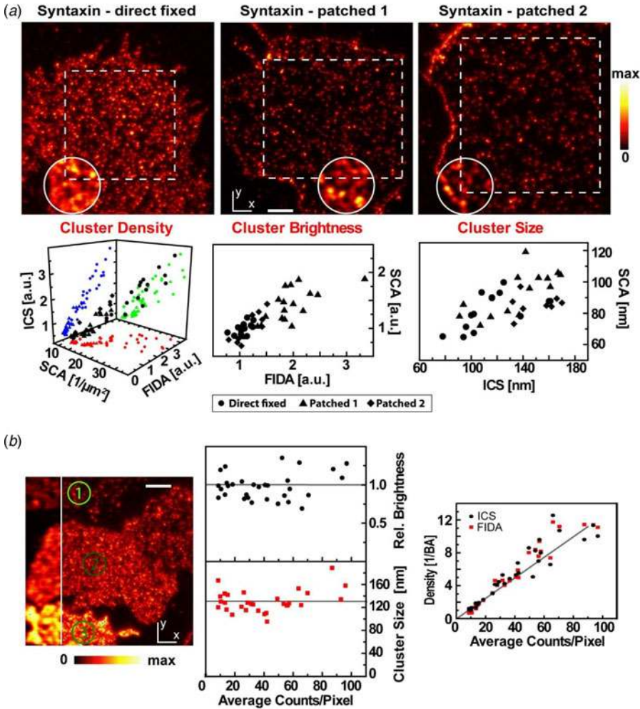
Fig. 5. STED nanoscopy: Cluster analysis. (a) ICS, FIDA and SCA analysis of syntaxin clusters recorded by STED. Upper panels: STED and confocal (circled areas) images of membrane sheets of PC12 cells immunolabeled for syntaxin for three different preparations (directly fixed (left) and patched 1 (middle) and 2 (right)). For the latter two, clustering is reinforced and cluster density decreased, dashed rectangles: analysed area, scale bar: 500 nm. Lower panels: values of cluster density (left), brightness (middle) and size (right) determined for different cells of the different preparations (dots: direct fixed, triangles: patched 1, diamonds: patched 2); left panel: 3D data (black) and projections to different value pairs (blue, green, red) of cluster density by ICS, FIDA and SCA, showing agreeing results by the different analysis techniques. (b) Syntaxin cluster morphology is independent of its expression level. Left panel: STED and confocal (left part) image of three representative membrane sheets generated from PC12 cells expressing different levels of immunolabeled myc syntaxin 1A (cell 1 with a low (probably endogenous) level of syntaxin, and cells 2 and 3 with different overexpression levels, adapted from (Sieber et al. 2006)). Plot of cluster brightness (upper middle), size (lower middle) and density (right) against the expression level ( \sim average pixel brightness) determined by ICS (black) and FIDA (red) from the STED images of different cells, revealing no variation of brightness and size with expression level, and a linear increase of density with expression level.
