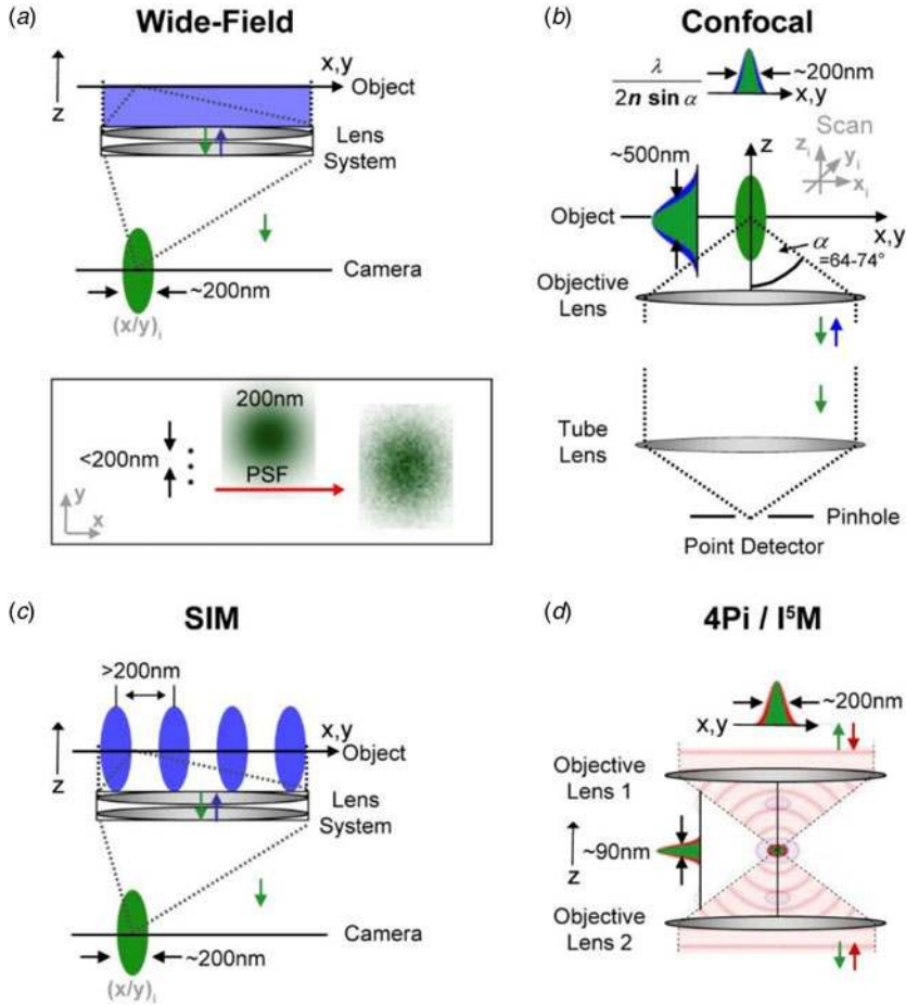
Fig. 1. Diffraction-limited far-field fluorescence microscopy. An object is illuminated with excitation light (blue) and its fluorescence (green) imaged onto a detector using a lens system, whereby the object is placed > \mu\text{m} away from any optics. (a) In a wide-field microscope a large area of the object is illuminated at once and signal imaged onto a camera. (b) In a point-scanning confocal microscope a diffraction-limited volume is illuminated, signal detected on a point-detector through a pinhole, and the final image formed by scanning the spot over the object. The size of the focused and observed spot is governed by the focusing strength of the objective lens (given by the angle \alpha ), the wavelength \lambda of the applied light, and the refractive index n of the object medium. Bax: Due to the focusing of light one cannot image point-like objects to dimensions smaller than approximately 200 nm in the lateral ( x,y ) and 600 nm in the axial ( z ) directions for visible light. This finite-sized, diffraction-limited point spread function (PSF) precludes the discerning of alike objects closer together than these 200 nm and results in blurred images at these spatial scales. Different versions of far-field microscopy have been implemented with the goal to push the diffraction barrier to its limits. (c) A two-fold increase in spatial resolution has been realized by SIM using, for example, a standing wave pattern in a wide-field mode with the pattern maxima separated by more than the 200 nm. (d) Using two opposing objective lenses for illumination and/or detection, the axial resolution of a wide-field or point-scanning/confocal microscope can be enhanced multi-fold, denoted I 5 M or 4Pi, respectively. (Here, red: excitation, and green: fluorescence)
