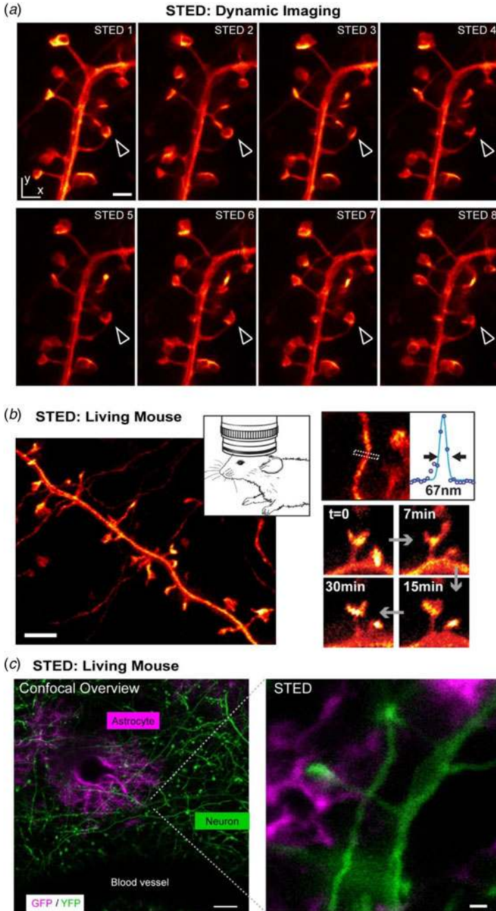
Fig. 6. Live-cell STED nanoscopy. (a) Time-lapse STED imaging of dendritic processes in a living hippocampal slice culture labeled with the fluorescent protein YFP (1 frame every 40 s, adapted from (Nägerl et al. 2008)). Arrows indicate a change in shape over time of a cup-like spine head. Scale bar: 1 \mu\text{m} . (b) In-vivo STED nanoscopy of a YFP-labeled neuron in the molecular layer of the somatosensory cortex of a mouse (left, inset depicts imaging setup). A maximum intensity projection of dendritic and axonal structures proves a spatial resolution of <70\text{ nm} (upper right). Temporal dynamics of spine morphology (lower right). Scale bar: 1 \mu\text{m} . Adapted from (Berning et al. 2012). (c) Two-color in-vivo STED imaging of astrocytes and neurons offers the possibility to study the influence of the astrocyte on
