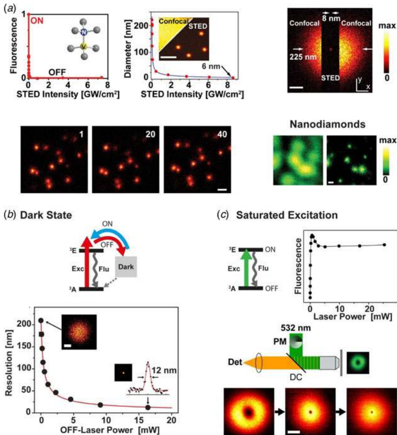
Fig. 11. The resolution of coordinate-targeted nanoscopy is in principle limited only by the size of the quantum system (molecule or emitter) to be distinguished: imaging nitrogen-vacancy (NV) centers in diamond. (a) STED imaging of NV centers. (Upper left) NV centers (inset: molecular structure) are a nearly perfect switch: fluorescence inhibition versus STED laser intensity. (Upper middle) STED images of single isolated NV centers in bulk diamond (inset: scanning image, with confocal counterpart in the upper left corner) reveal down to 6 nm spatial resolution (or diameters of the observation area) with increasing STED laser intensity. Scale bar: 100 nm. (Upper right) Scanning image of a single isolated NV center (fast axis along y ) with STED laser switched on only in the marked area, exemplifying the vast increase in spatial resolution from confocal 225 nm down to 8 nm. Scale bar: 100 nm. (Lower left) Repetitive STED images of single isolated NV centers in diamond (frame number in the upper right corner), showing the ultimate stability of these emitters. Scale bar: 200 nm. (Lower right) Confocal (left) and STED (right) images of 35 nm large NV-containing nanodiamonds. Scale bar: 100 nm. Adapted from (Han et al. 2009; Rittweger et al. 2009a). (b, c) GSD nanoscopy of NV centers. (b) GSD by reversible laser-driven transitions into a long-lived dark state. (Upper panel) Energy level diagram of an NV center with ground 3 A, excited 3 E and dark states, transitions driven by red (excitation Exc and OFF-switching) and blue light (ON-switching), spontaneous fluorescence emission (Flu) and dark state return (dashed line, >100 s lifetime). (Lower panel) Spatial resolution versus power of the red laser driving the OFF transition, as determined by scanning images of isolated NV centers and respective intensity line profiles (insets, scale bar is 100 nm). Adapted from (Han et al. 2010). (c) GSD by saturated excitation. (Upper left panel) Energy level diagram of an NV center with 3 A (OFF) and 3 E (ON) states, and excitation by green light (Exc) and spontaneous fluorescence emission (Flu). (Upper right panel) Saturation of fluorescence signal: dependence of fluorescence signal of a single NV center on the power of the excitation laser. (Middle panel) Experimental setup with green 532 nm excitation laser, phase plate (PM) generating the doughnut-shaped intensity distribution (inset), dichroic mirror (DC), fluorescence signal (orange), and detector (Det). (Lower panels) Scanning images of a single NV center for increasing intensity of the excitation laser (left to right), depicting the confinement of the area in which no fluorescence is elicited. Adapted from (Rittweger et al. 2009b). Scale bar: 50 nm.
