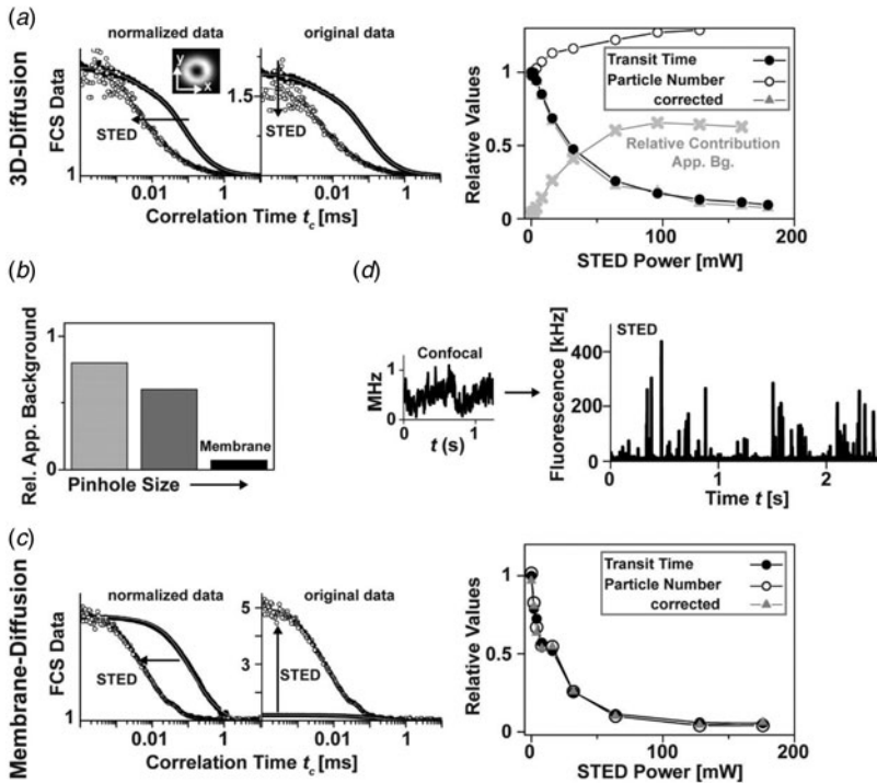
Fig. 8. STED-FCS. (a) STED-FCS analysis of free 3D-diffusion of the organic dye Atto647N in aqueous solution. Representative correlation data (left panels, left: normalized amplitudes, right: original data) for confocal (black) and STED recordings (open dots) and (right panel) relative values of transit time \tau_D (black), particle number N (original open dots, background-corrected grey triangles), and signal fraction of apparent background (grey crosses) determined from FCS and FIDA data recorded for increasing power of the doughnut-shaped (inset left) STED laser. The size reduction of the observation spot by increasing the STED power shortens the dye's transit time, but also introduces an increasing contribution of apparent un-depleted low-brightness background, which introduces noise and dampens the FCS data's amplitude and thus results in an apparent increase of N , which can be corrected for by a global FCS-FIDA analysis. (b) Relative apparent background for the STED-FCS recordings for two different pinhole sizes (decrease from left to right), and for a fluorescent lipid analog diffusing in a multi-lamellar membrane. Reduction of the pinhole size reduces un-depleted out-of-plane low-brightness fluorescence signal (apparent background), which diminishes further when measuring two-dimensional diffusion in membranes, where out-of-plane signal is absent. (c) STED-FCS analysis of free 2D-diffusion of a fluorescent lipid analog in a multi-lamellar membrane. Representative correlation data (left panels, left: normalized amplitudes, right: original data) for confocal (black) and STED recordings (open dots) and (right panel) relative values of transit time \tau_D (black) and particle number N (original open dots, background-corrected grey triangles) determined from FCS and FIDA data recorded for increasing power of the doughnut-shaped STED laser. The confinement of the observation spot by increasing the STED power reduces both \tau_D and N , without an influence by out-of-plane signal contributions. (d) STED allows single-molecule observations at high concentrations. Fluorescence signal over time for the same concentration of a fluorescent lipid analog diffusing in a multi-lamellar membrane indicates diffusion of single molecules only for the STED (right) but not for the confocal (left) recordings. Adapted from (Ringemann et al. 2009).
