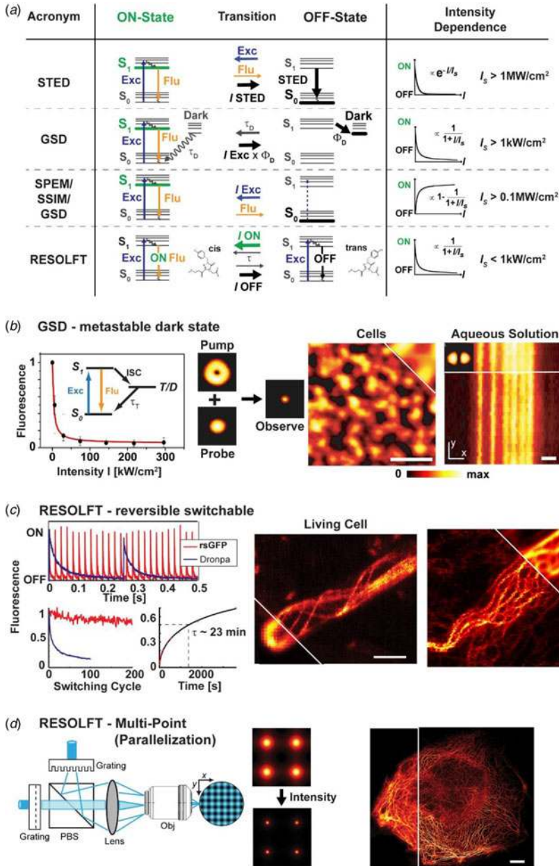
Fig. 10. Generalization of coordinate-targeted (deterministic) nanoscopy: the RESOLFT concept. (a) Different molecular states and transitions can be applied to reversibly inhibit fluorescence for coordinate-targeted nanoscopy ranging from STED (stimulated emission), over GSD (metastable dark states), SPEM/SSIM/GSD (ground state depletion by saturated excitation) to RESOLFT (e.g. photoswitchable fluorophores, different conformational states): acronyms (left), molecular states (middle) with energy level diagram of a fluorophore (ground S_0 , excited S_1 and dark states) and transitions for ON (left middle) and OFF (right middle) direction (middle: ON-OFF transitions with excitation (Exc), fluorescence (Flu), stimulated emission (STED), metastable dark states (with crossing probability \Phi_D and lifetime \tau_D ), bright (ON) and dark (OFF) conformational states (with on- and off-switching light and potential spontaneous transition lifetime \tau ) and intensity I of the corresponding lasers), intensity I dependence of switching with threshold intensities I_S (right), and approximate values of I_S . Adapted
