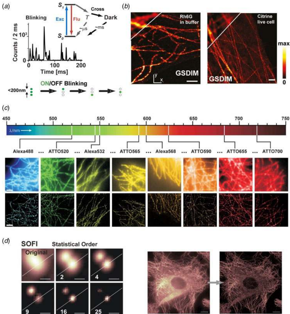
Fig. 13. Coordinate-stochastic single-marker/single-molecule switching: stochasticity in space and time (GSDIM, (d)STORM, ...) and SOFI. (a) A fluorophore can continuously be cycled between its bright singlet ( S_0 and S_1 , emitting fluorescence (Flu)) and dark state (triplet T and other long-lived ( \mu\text{s} - \text{ms} ) dark states) system with a single excitation (Exc) laser, eliciting on-off blinking of fluorescence in time (as highlighted by a fluorescence time trace of a single Atto532 fluorophore in PVA, adapted from (Fölling et al. 2008b)) and space (as sketched in the lower panel for three different single molecules). (b) GSDIM/(d)STORM/... images of Rh6G-immunostained microtubules in PtK2 cells in aqueous buffer (left) and of the microtubule cytoskeleton of living PtK2 cells labeled with the fluorescent protein Citrine-Map2 (right). Upper left corner: Diffraction-limited wide-field recordings. Scale bars: 1\ \mu\text{m} . Adapted from (Fölling et al. 2008b). (c) GSDIM/(d)STORM/... allows the use of a whole gamut of conventional organic dyes with different emission spectra as highlighted by super-resolution (lower panels) and corresponding diffraction-limited wide-field (upper panels) images of the cytoskeletal network of mammalian cells immunolabeled with eight different Alexa Fluor and Atto dyes spanning the visible wavelength range (emission maxima in upper color bar) according to the dSTORM principle (scale bar: 1\ \mu\text{m} , adapted from (Heilemann et al. 2009b)). (d) Principle of SOFI imaging. SOFI is based on higher-order statistical analysis of temporal fluctuations recorded in a sequence of images. The spatial resolution increases with the order as exemplified by SOFI images of different order (as indicated) of two blinking quantum dots deposited on a cover slip (left, scale bars: 250\ \text{nm} , adapted from (Dertinger et al. 2009)). (Right) Diffraction-limited wide-field (left) and SOFI (right) images of quantum-dot immunolabeled tubulin network of a 3T3 fibroblast (scale bar: 10\ \mu\text{m} , adapted from (Dertinger et al. 2010)).
