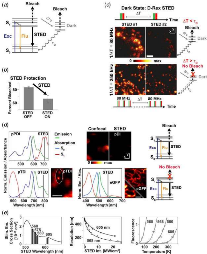
Fig. 4. STED nanoscopy: photophysics and bleaching. (a) Photobleaching pathways: excitation (Exc) elevates a fluorophore from its ground S_0 to its first excited electronic state S_1 , from where it either returns to S_0 by spontaneous fluorescence emission (Flu) or by STED, or it traverses with probability \Phi_D to a dark state whose lifetime \tau_D (time before return to S_0 ) is much longer than that of S_1 . Photobleaching may occur from S_1 and the dark state, and is most pronounced from higher excited electronic states after further absorption of excitation or STED light (higher-order photobleaching, dashed lines). Horizontal lines: electronic states (thick) and vibrational sub-states (thin). Curved lines: vibrational transitions. (b) Suppression of photobleaching rate by STED: stimulated emission shortens the lifetime of S_1 and thus the probability of photobleaching as exemplified by the percentage of signal bleached after scanning a layer of the organic dye KK114 with and without the addition of STED light (excitation at 488 nm with 9 kW/cm 2 and STED at 760 nm with 0.8 GW/cm 2 , repetition rate 76 MHz, scanning dwell time 10 ms). (c) Higher-order photobleaching from long-lived dark states, as exemplified by subsequent scanning STED images of 40-nm sized fluorescent beads, showing a significant loss of signal due to irreversible photobleaching (upper images). D-Rex illumination, i.e. increasing the time \Delta T between subsequent pairs of excitation and STED pulses (i.e. decreasing the repetition rate 1/\Delta T ) above the dark states lifetime \tau_D allows the dark states to relax before incidence of the next pulses, avoiding higher-order photobleaching (lower images). D-Rex illumination by fast beam scanning (lower panel): for a fluorophore the incidence of only a few excitation-STED pulse pairs of high repetition rate (e.g. 80 MHz) is followed by a long resting period \Delta T until the scanned beam pair hits the same spot again. (d) Higher-order photobleaching from the first excited electronic state S_1 , as exemplified for the organic dyes pDI and pTDI and for eGFP. Absorption spectra of S_0 (blue) and S_1 (red) and fluorescence
