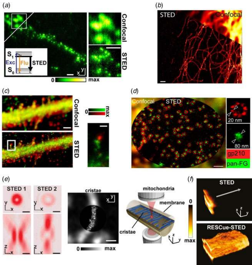
Fig. 3. STED nanoscopy. (a) A reversible molecular transition is realized by stimulated emission (inset): the turn-on light excites (Exc) the fluorophores from their (dark) ground S_0 to their (bright) excited S_1 state, where de-excitation by spontaneous fluorescence emission (Flu) is overruled by the addition of the STED laser inducing stimulated emission. Example scanning STED nanoscopy image of fluorescently labeled synaptotagmin I in fixed cultured hippocampal neurons, exemplifying the superior spatial resolution over conventional confocal microscopy and revealing that this protein is clustered in isolated patches on the presynaptic plasma membrane after synaptic vesicle exocytosis (adapted from (Willig et al. 2006c)). Scale bar: 1 \mu\text{m} . (b) Confocal (upper right) and STED images of immunolabeled microtubules in fixed mammalian cells (adapted from Wurm et al. 2012). Scale bar: 500 nm. (c) Multi-color STED nanoscopy determining the co-localization of different molecules with sub-diffraction resolution, as exemplified for the D1 dopamine receptor and Na 1 K 1 -ATPase in cultured striatal neurons (lower image: confocal recording, adapted from (Blom et al. 2012)). Scale bars: 1 \mu\text{m} (in enlarged image: 200 nm). (d) Multi-color STED and confocal (peripheral parts) recordings of immunolabeled subunits in amphibian nuclear pore complexes (NPCs) of cultured Xenopus cells with close-ups (right) of the spatial organization of the peripheral gp210 and central pore pan-FG proteins in a single NPC (adapted from Göttfert et al. 2013). Scale bar: 500 nm. (e) 3D STED nanoscopy realized by overlapping two STED beams featuring confinement along the lateral x/y and axial z direction, respectively (left: x - y (upper) and x - z (lower) projections of the intensity distributions of the two STED lasers, scale bars: 200 nm), and by the use of two opposing microscope objectives (O1 and O2, right). The resulting isotropic observation spot of diameter below 40 nm allows the recording of super-resolved 3D images, as exemplified by resolving mitochondrial cristae (middle, scale bar: 1 \mu\text{m} , adapted from (Schmidt et al. 2009)). (f) RESCue STED: Reduction of photobleaching in 3D STED imaging by applying an intelligent light exposure scheme that minimizes the number of excitation/de-excitation events a fluorophore has to undergo during recording of a scanning image: conventional (upper) and RESCue (lower) 3D STED
