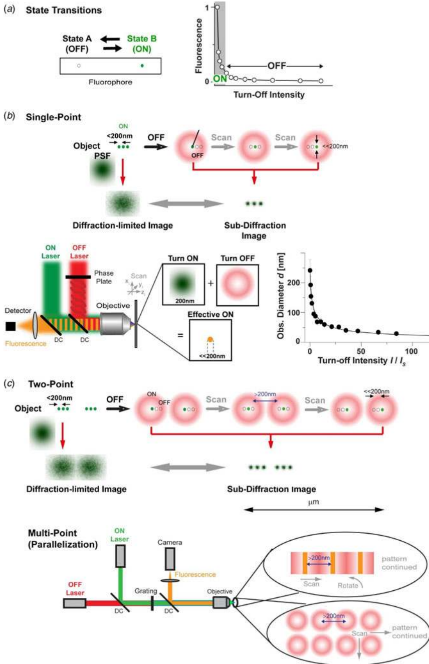
Fig. 2. Sub-diffraction imaging by the coordinate-targeted (deterministic) approach (STED/RESOLFT): driving molecular transitions in space. (a) Sub-diffraction imaging is based on reversibly inducing transitions between molecular states of different fluorescence emission properties (such as a bright ON- and a dark OFF-state), where at least one of the transitions such as the ON-to-OFF transition is driven by light (left). Increasing the intensity of the turn-off light above a certain threshold turns off the fluorescence emission (right). (b) In its single-spot scanning version the diffraction-limited spot of the fluorescence excitation or turn-on laser (green) is overlaid with an additional turn-off laser which features a central intensity zero (red). Increasing the intensity I of the turn-off laser far above a threshold value
