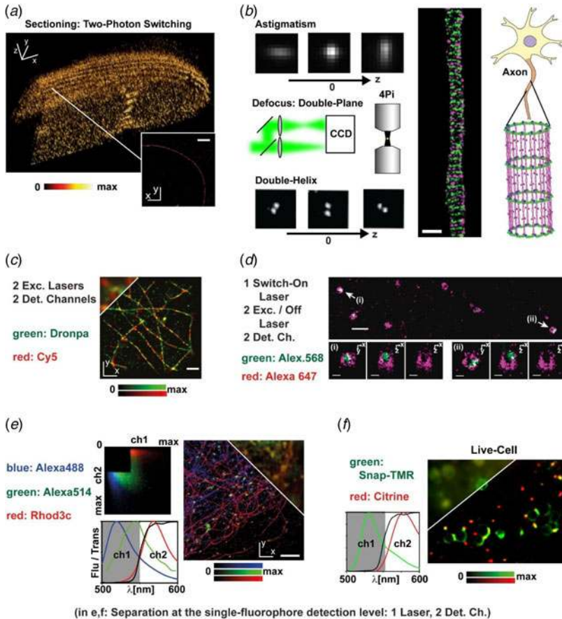
Fig. 14. 3D and multi-color imaging with coordinate-stochastic single-marker/single-molecule switching-based nanoscopy. (a) Optical sectioning and out-of-plane signal rejection achieved by two-photon on-switching or activation: Super-resolution images of lamin of a U373MG cell stained with a photoactivatable rhodamine (inset: equatorial slice as marked by the line, scale bar: 2 \mu\text{m} , adapted from (Fölling et al. 2007)). (b) (Left) Different approaches of 3D (F)PALM/STORM-based imaging: astigmatism using a cylindrical lens results in an elliptical distortion of the images of out-of-plane (axial z -direction) molecules, double plane imaging comparing focused and defocused camera images, 4Pi using two opposing objectives, and double-helix detection employing a ‘doubled’ detection of each single molecule where the orientation of the two lobes of intensity changes with the z -position of the molecule. (Right) Two-color STORM image of immunolabeled bII-spectrin (green) and adducin (magenta) in fixed axons reveals that actin, spectrin and adducin form a coordinated, quasi-1D lattice structure in axons (scale bar: 500 nm, adapted from (Xu et al. 2013), where 3D astigmatic imaging was also performed). (c) Two-color image of the microtubular network in a PtK2 cell stained with the reversibly photoswitchable protein rsFastLime (green) and the organic dye Cy5 (red) generated by subsequent recordings using two excitation lasers and two detection channels (upper left corner: diffraction-limited wide-field recording, scale bar: 1 \mu\text{m} , adapted from (Bock et al. 2007)). (d) Fast two-color 3D-STORM images of live BSC-1 cells using one activation and two excitation lasers inducing fluorescence blinking over time: Alexa 568-labeled transferrin (green) and clathrin-coated pits labeled with Alexa647 via a SNAP tag (magenta), x/y -projection of the recordings of multiple sections along z (upper panel), and different cross-sections through two objects (i, ii) indicated in the upper panel ( x/y near the plasma membrane (left), x/z cutting through the middle of the invaginating pits (middle) and corresponding x/z cross-section of the clathrin channel only (right)). Scale bars: 500 nm (upper panel) and 100 nm (lower panels), adapted from (Jones et al. 2011). (e, f) Multi-color imaging via single-molecule signatures using one continuously running laser and two detection channels. Color separation is realized by applying fluorescence labels with slightly
