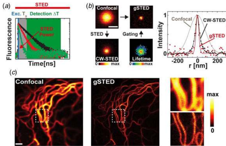
Fig. 7. gSTED nanoscopy. (a) Principle: the fluorescence lifetime of a fluorophore decreases with increasing STED power as depicted for representative fluorescence lifetime decays for different STED powers (left): using pulsed excitation (blue, Exc) and CW-STED (red) in conjunction with gated detection (detection within the time period \Delta T (green) with a time lag T_g (grey) relative to the exciting pulse) favors signal from points of low STED power, i.e. from areas at or close to the intensity zero. (b) Scanning fluorescence intensity (left and upper right) and lifetime (lower right) images of a single fluorophore for confocal diffraction-limited (upper left), CW-STED (intensity: lower left, lifetime: lower right) and gSTED (upper right) recordings (scale bar: 200 nm), and (right panel) intensity line profiles through the middle images, indicating the removal of the pedestal of the CW-STED recordings (black) by the gated detection (gSTED, red). (c) Confocal and gSTED images (right: magnification of central area marked by the dashed white box) of keratin fused to the fluorescent protein citrine in a living PtK2 cell with low CW STED laser power. Scale bar: 1 \mu\text{m} . Adapted from (Vicidomini et al. 2011).
