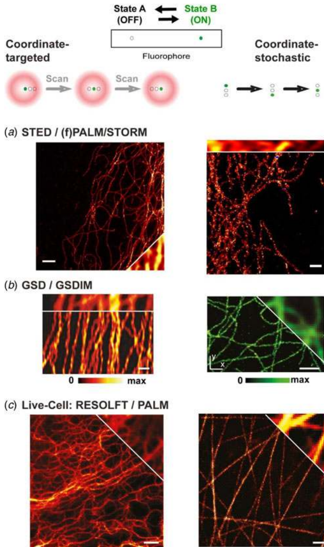
Fig. 15. Coordinate-targeted versus coordinate-stochastic nanoscopy. Both families of methods are based on transitions between molecular states of different fluorescence characteristics (such as a bright ON- and a dark OFF-state) realizing the separation of different molecules within a diffraction-limited area by subsequently confining emission either to sub-diffraction sized spots defined in space (coordinate-targeted (deterministic), left) or stochastically in space on single isolated molecules (coordinate-stochastic, right). Sub-diffraction coordinate-targeted and -stochastic imaging can be realized using the same fluorescence labels and switching mechanisms. (a) Coordinate-targeted STED (left) versus coordinate-stochastic (F)PALM/STORM images (right) of organic-dye-labeled microtubules in fixed PtK2 cells. (b) Coordinate-targeted GSD (left, scale bar 500 nm) versus coordinate-stochastic GSDIM images (right) of Atto532-labeled microtubules in fixed PtK2 cells. (c) Coordinate-targeted RESOLFT (left) versus coordinate-stochastic (F)PALM/STORM images (right) of the R5FP Dreiklang expressed in live PtK2 cells at Keratin19 (left) and Map2-microtubules (right). Adapted from (Brakemann et al. 2011). Diffraction-limited counterparts in upper parts. All other scale bars: 1 \mu m.
