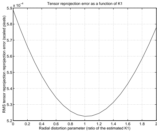
Figure 4: The tensor reprojection error as a function of the value of the radial distortion K1 .
