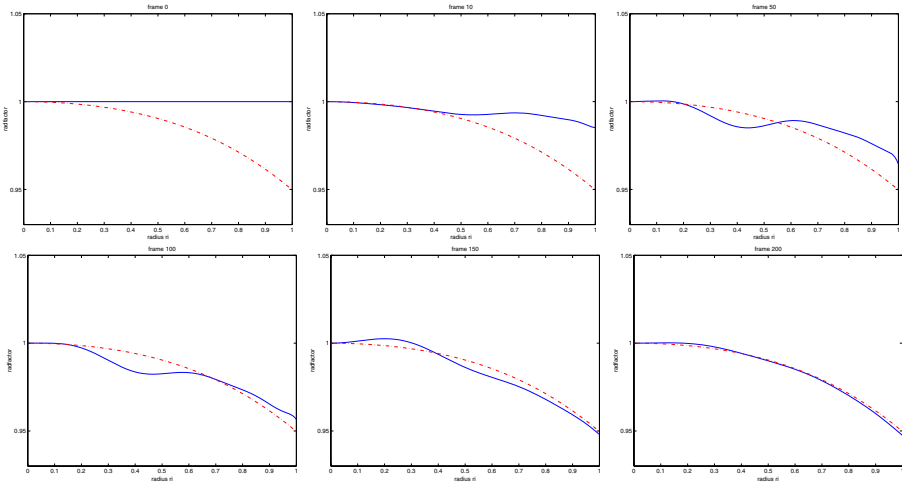
Fig. 6. From left to right [frames 0,10,50,100,150 and 200]: The convergence of the estimated radial factor (solid curve) towards the ground truth (dash-dot). The abscissa represents the radius in the ideal image plane \Pi_i . The ordinate represents the radial distortion factor radfactor .
