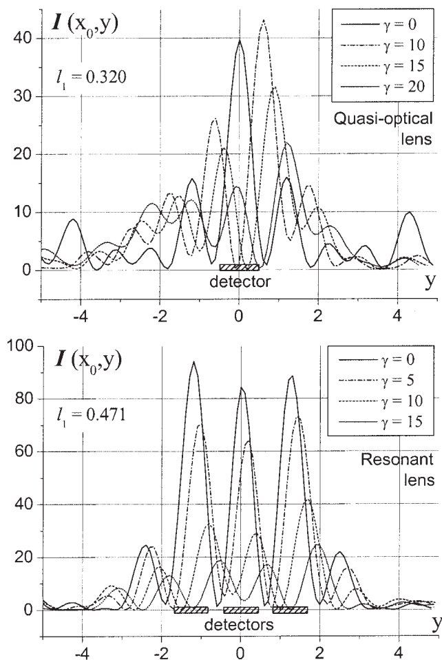
Figure 6 Field intensity along the flat sides of two differently extended lenses for a varying angle of the plane wave incidence (see insets): x_0 = al_1 , \epsilon = 11.7 , ka = 10 , l_2 = 1.0457
