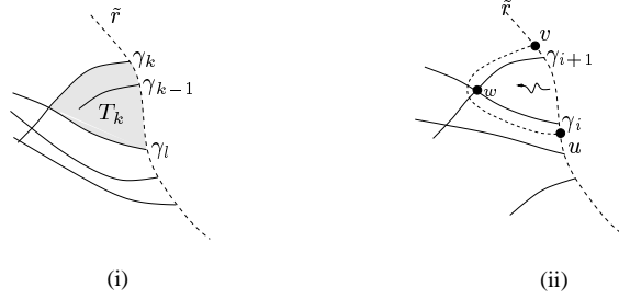
Figure 9. (i) e_l and e_k have a common endpoint counterclockwise to \tilde{r} ; (ii) advancing the sweep curve.
