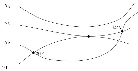
Figure 5. Edges of G with partially overlapping projections.
