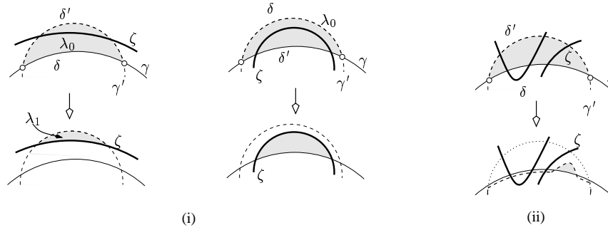
Figure 10. (i) Replacing \lambda_0 by a “smaller” lens if it intersects a type (i) curve. (ii) Shrinking \lambda_0 to an empty lens when it is crossed only by type (ii) curves.
