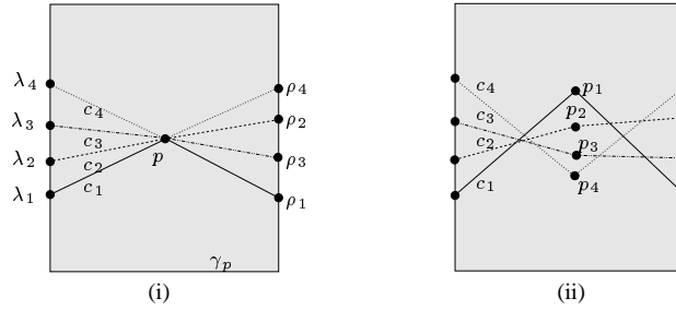
Figure 11. Perturbing arrangements in degenerate position: (i) Straightening the curves in the vicinity of a degenerate point p . (ii) Deforming the curves near p . (Note that c_2 and c_3 cross at p , while every other pair is tangent at p .)
