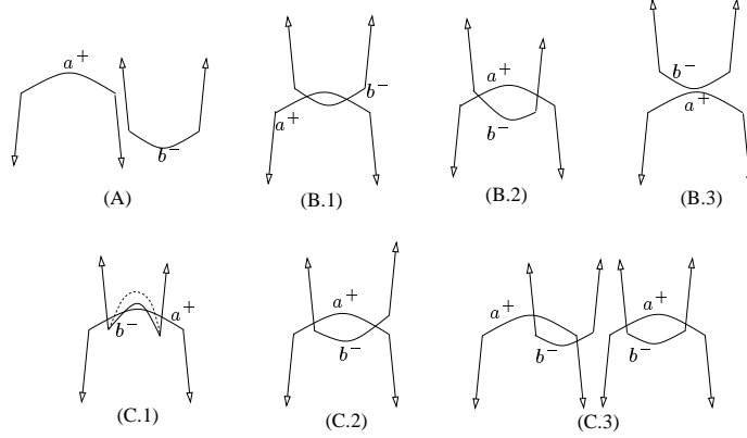
Figure 19. An extended upper arc and an extended lower arc intersect at most twice: (A) \rho_a lies to the left of \lambda_b ; (B) \lambda_b lies above a^+ : (B.1) a^+ , b^- intersect at two points; (B.2) a^+ and b^- intersect at one point; (B.3) a^+ and b^- do not intersect. (C) \lambda_b lies below a^+ : (C.1) a^+ and b^- intersect at two points (an impossible configuration); (C.2) a^+ and b^- intersect at one point; (C.3) a^+ and b^- do not intersect.
