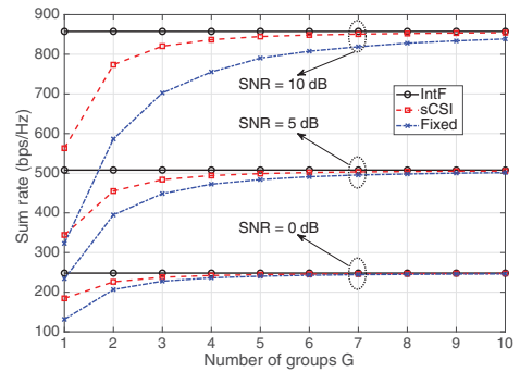
Fig. 2. Sum rate performance of SAUG with different transmission approaches versus the number of scheduled UT groups when FFR is adopted.
