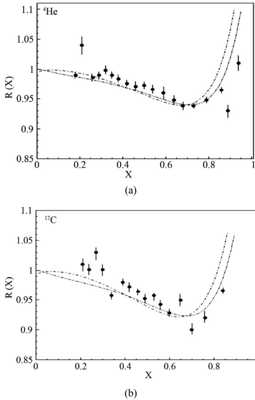
Figure 2. The R_{EMC}^A(x) for {}^4\text{He} and {}^{12}\text{C} nuclei are plotted. We use two different nucleon structure functions. One of them is nucleon structure function based on GRV nucleon structure function of free proton and neutron [12] i.e. dashed and the other have been taken from Ref. [5] i.e. dash-double dotted. The experimental data have been taken from Ref. [19].
