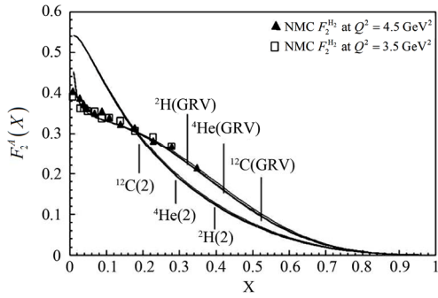
Figure 1. The structure function of {}^2\text{H} , {}^4\text{He} and {}^{12}\text{C} nuclei. In order to obtain the nucleus structure function we have used the GRV structure function of the free proton. The experimental data are taken from [15,16].
