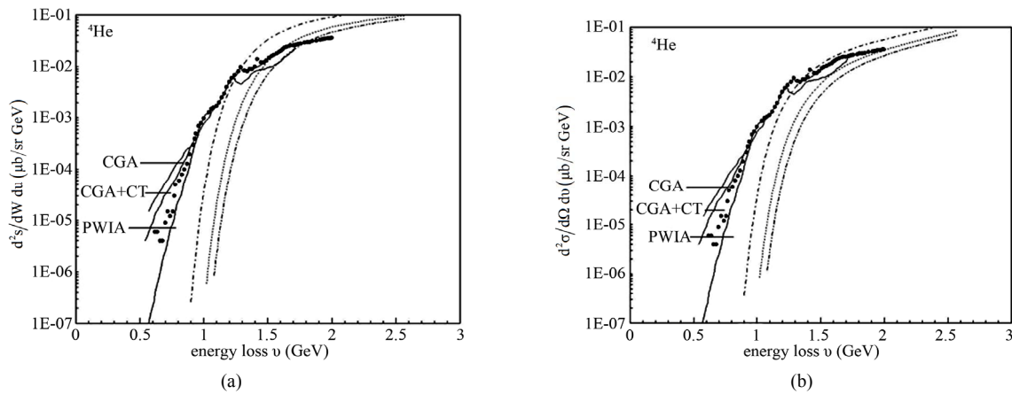
Figure 3. The (a) and (b) diagrams show the deep inelastic cross section of electron beam from ^4\text{He} nuclei. We have used the GRV nucleon structure function [12] for calculation of nucleus structure function that plotted in (a) and nucleon structure function from [5] for calculating of nucleus structure function that plotted in (b) diagram. The dash-double-dotted and dot and dash-dotted curves shows our calculation. The CGA, CGA + CT, PWIA curves, and experimental data have been taken from [22].
