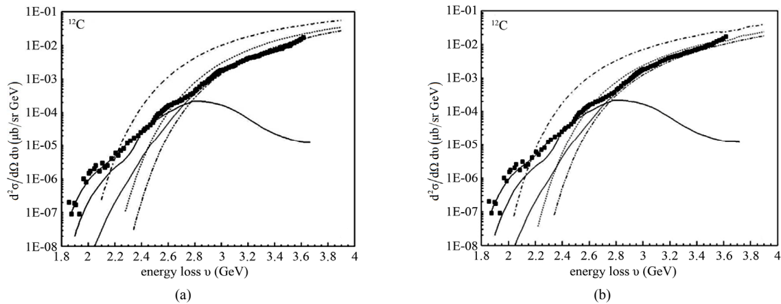
Figure 4. The (a) and (b) diagrams show the deep inelastic cross section of electron beam from ^{12}\text{C} nuclei. We have used the GRV nucleon structure function [12] for calculation of nucleus structure function that plotted in (a) and nucleon structure function from [5] for calculating nucleus structure function that plotted in (b) diagram. The three full curves and experimental data have been taken from [23].
