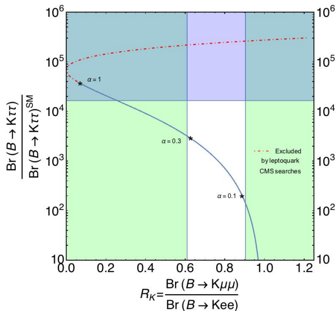
Figure 2. Prediction of MLFV to first order in lepton Yukawas in the form of a line in the plane of R_K vs \mathcal{B}(B \rightarrow K\tau\tau) , the experimentally allowed region at 90% CL is the white band. In the case in which the effect is produced by a hypercharge-2/3 leptoquark and applying MFV in the quark sector too, CMS direct searches exclude the red dashed part of the line. The points marked with \alpha \equiv g^2/(4\pi) = 1, 0.3, 0.1 correspond to the prediction for a 600 GeV leptoquark with the coupling constant defined in eq. (6.6).
