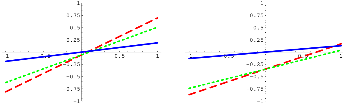
Fig. 170: As in Fig. 169, except for the value of b ; here b = 7 .
