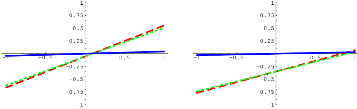
Fig. 169: I plot here 1 - R_{<sup>U</sup>}^C (red long-dashed line), 1 - R_{<sup>C</sup>}^C (green short-dashed line), and R_{<sup>C</sup>}^C - R_{<sup>U</sup>}^C (blue solid line) as a function of \beta , for a = 4, b = 4.5 , and \alpha = 0.1 (left panel) or \alpha = 0.9 (right panel).
