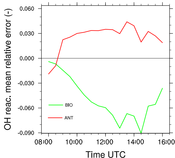
Figure 10. Mean relative error E_{\text{ROH}} made on the OH reactivity by neglecting turbulent motions for the biogenic case (green) and the anthropogenic case (red).
