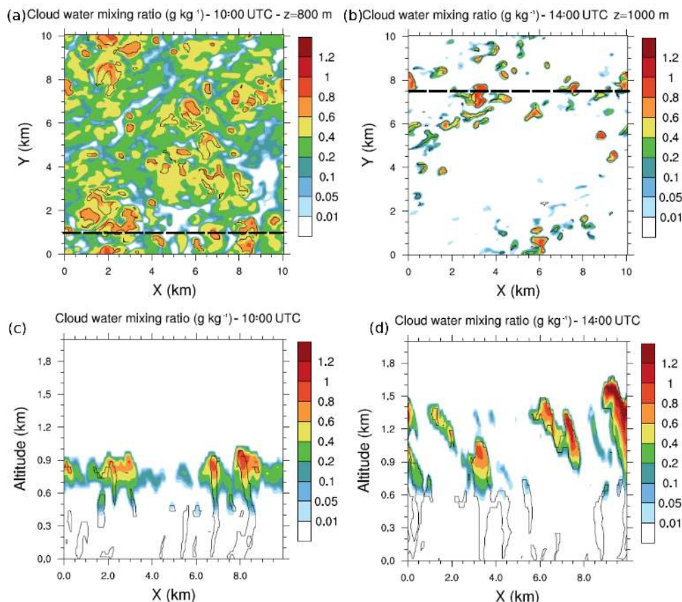
Figure 2. (a) Cloud water mixing ratio horizontal cross sections at 10:00 UTC and 800 m height and (b) at 14:00 UTC and 1000 m height. Black dashed lines represent the vertical cross sections at (c) 10:00 UTC and y = 1 km and at (d) 14:00 UTC and y = 7.5 km. Black isolines denote thermals identified by the conditional sampling method.
