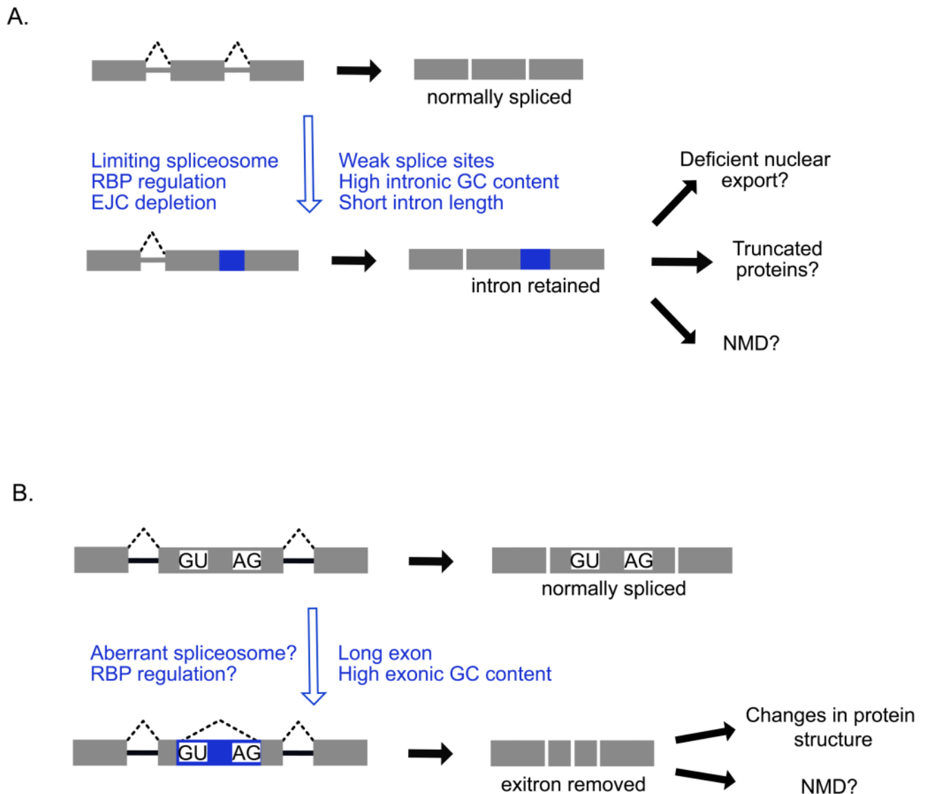
Figure 3. Intron retention and exons.
