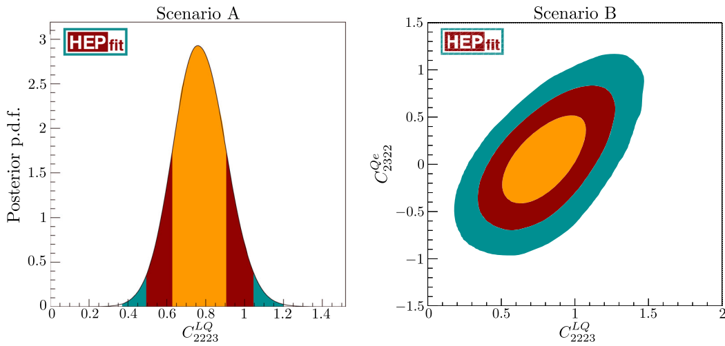
FIG. 3. Left panel: posterior probability density function (p.d.f.) for the NP coefficient C_{2223}^{LQ} in scenario A. Right panel: joint posterior p.d.f for C_{2223}^{LQ} and C_{2322}^{Qe} in scenario B. We show 68%, 95% and 99.7% probability regions in orange, red and green respectively. All results are obtained using the parametrization of hadronic contributions in Eq. (6).
