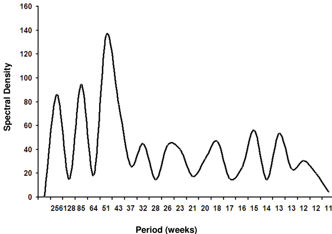
Figure 1 Periodogram Constructed from Spectral Decomposition of Weekly Pneumococcal Case Counts. Spectral density is represented on the y-axis, and can be conceptualized as a measure of goodness-of-fit for oscillatory regression models at different frequencies. The large peak at a frequency of 51 weeks suggests that invasive pneumococcal disease is a process that oscillates with annual periodicity (and is, in other words, compatible with wintertime seasonality). The two peaks at lower frequencies are lower harmonics illustrating bi- and tri-annual behaviour.
