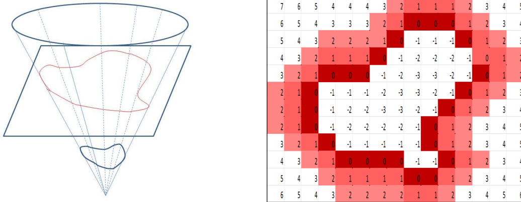
Fig 1: The Level Set Visualization
