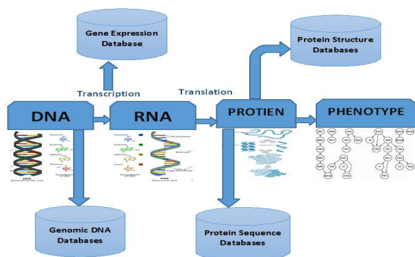
Fig. 15 Bioinformatics Types
