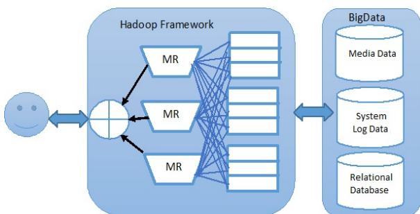
Fig. 6 Framework of Hadoop
