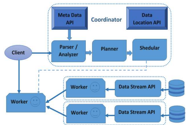
Fig. 11 Presto Architecture
