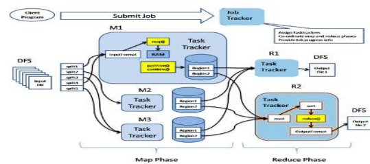
Fig. 8 MapReduce Architecture
