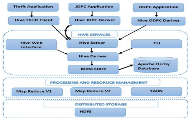
Fig. 9 Hive Architecture
