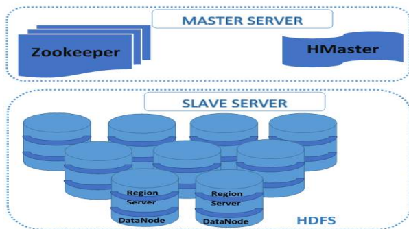
Fig. 10 Hbase Architecture
