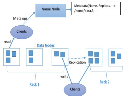
Fig. 7 Architecture of HDFS
