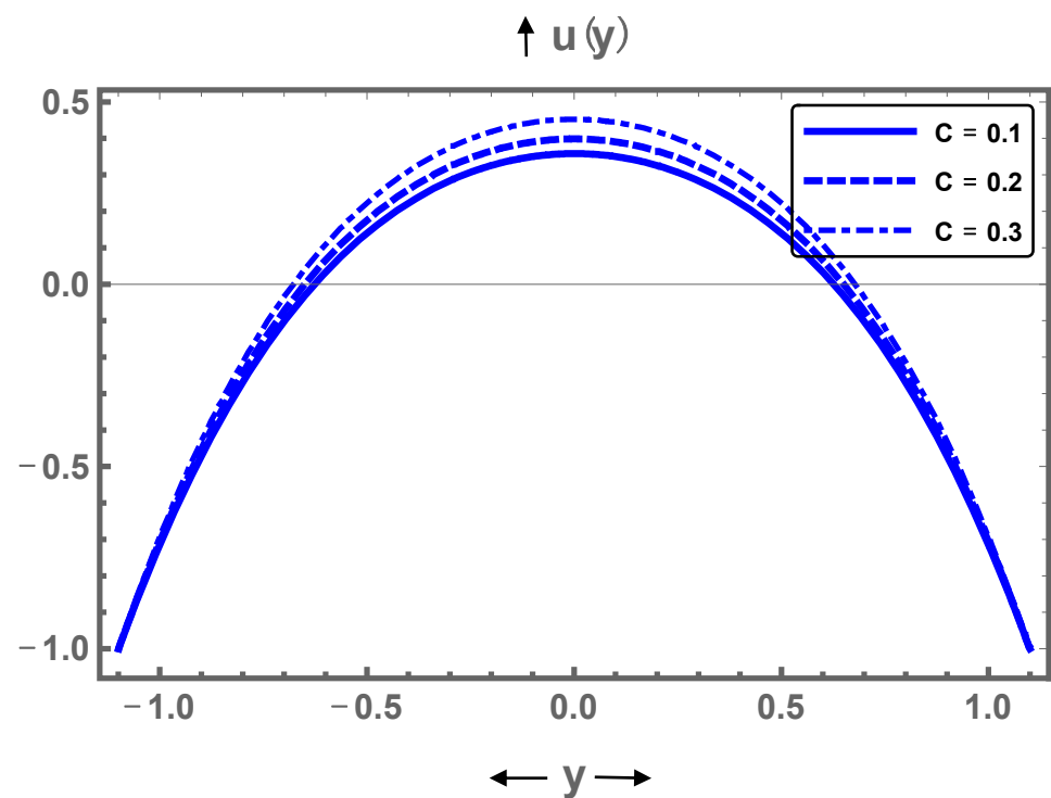
Figure 13. Display of axial velocity for different values of C .
