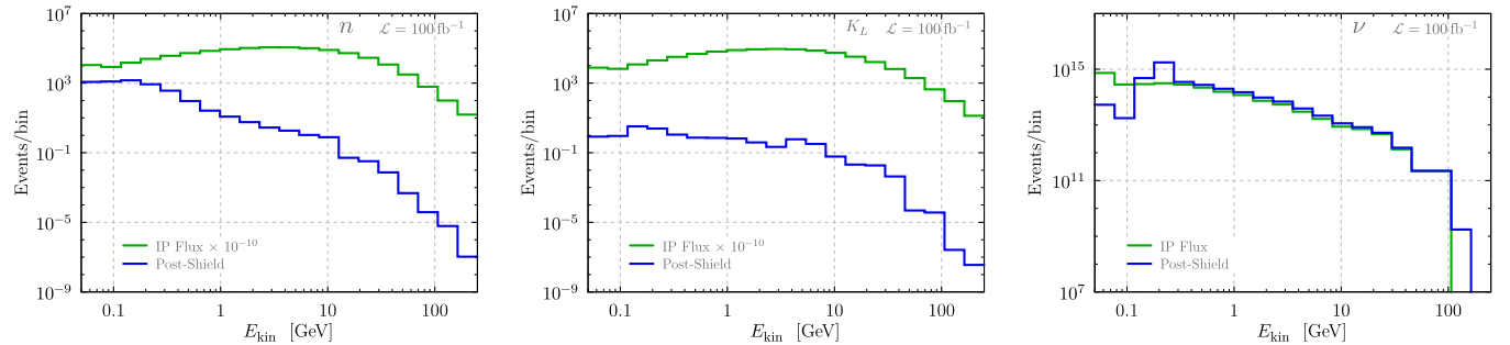
FIG. 3. Kinetic energy spectra of outgoing neutrons, K_L 's and neutrinos (blue), compared to their fluxes from the IP (green). For the sake of visual clarity, both the neutron and K_L fluxes from the IP are scaled by a factor of 10^{-10} .
