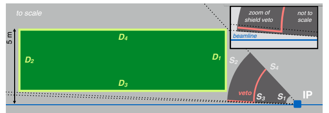
FIG. 2. Configuration of the shield, to scale.
