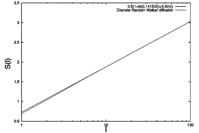
FIG. 1. Diffusion entropy of a random walker as a function of the number of jumps l . The dashed line and the solid line denote the discrete diffusion entropy S_d(l) , of Eq. (35) and the continuous prescription of Eq. (5), respectively. After a short transient the dashed line converges to the solid line.
