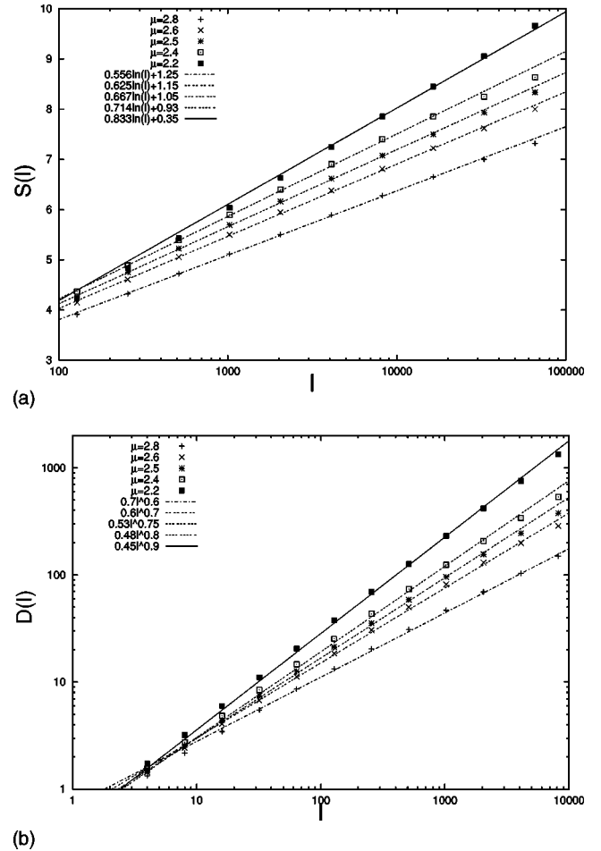
FIG. 3. Diffusion entropy and standard deviation of the Lévy process generated by artificial sequences \xi_i , corresponding, respectively, to five different values of the power coefficient \mu , namely, \mu=2.8, 2.6, 2.5, 2.4, 2.2 , and T=0 . The numerical results of the diffusion entropy analysis (DEA) (a) and of the standard deviation analysis (SDA) (b), reported as symbols, are in perfect agreement with the theoretical predictions, reported as fitting lines and obtained by using, respectively, the values of the probability distribution function scaling exponent \delta and of the exponents H in Table I.
