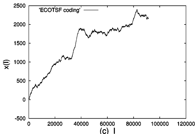
FIG. 4. In (a) we report the DNA walk relative to HUMTCRADCV, a noncoding chromosomal fragment. In (b) and (c), we report the DNA walk relative to ECO110K and ECOTSF, two coding genomic fragments.
