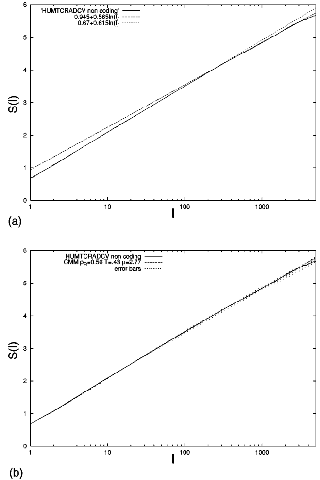
FIG. 7. Diffusion entropy for the HUMTCRADCV (the noncoding chromosomal fragment) and its CMM simulation. (a) shows that the DE analysis results in a scaling changing with time. The slope of the two straight lines is \delta' = 0.615 \pm 0.01 in the short-time region, and \delta = 0.565 \pm 0.01 in the long-time regime. (b) shows the comparison between the DEA of the real noncoding sequence and an artificial sequence corresponding to the CMM model: p_R = 0.56 \pm 0.02 , T = 0.43 , \mu = 2.77 \pm 0.02 .
