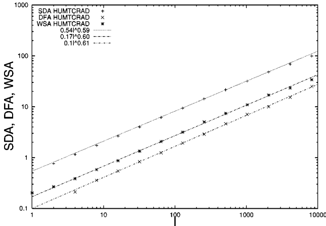
FIG. 5. Application of the three variance methods SDA, DFA, and WSA to the sequence HUMTCRADVC, the noncoding chromosomal fragment. The three methods give the same exponent H . In fact, we get H=0.59\pm 0.01 (SDA), H=0.60\pm 0.01 (DFA), and H=0.61\pm 0.01 (WSA), where the differences are within the error bars. Moreover, H is the same both at short time and long-time regions (i.e., H'=H ).
