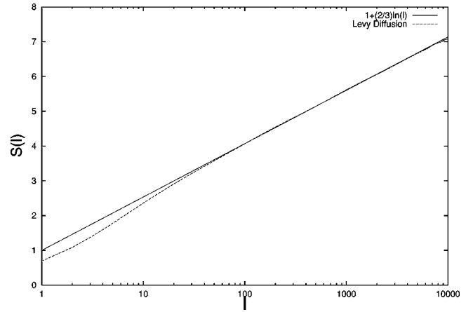
FIG. 2. Diffusion entropy of the Lévy process generated by an artificial sequence \xi_i , corresponding to the power coefficient \mu = 2.5 and T=0 . The dashed line is the diffusion entropy S_d(l) in the discrete-space perspective given by the Eq. (33). The solid line is the diffusion entropy S(l) in the continuous-space perspective given by Eq. (39). After an initial transient, the dashed line converges to the solid line.
