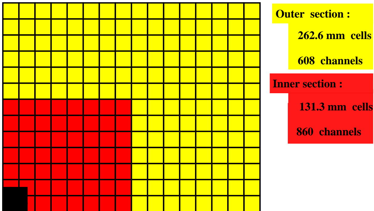
Figure 2.2: Lateral segmentation of HCAL. One quarter of the detector front face is shown.
