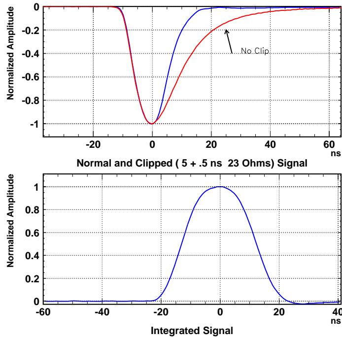
Figure 3.23: 80\text{ GeV} HCAL signals. The upper figure shows the PM signal before and after clipping, the lower one shows the same signal at the output of the integrator.
