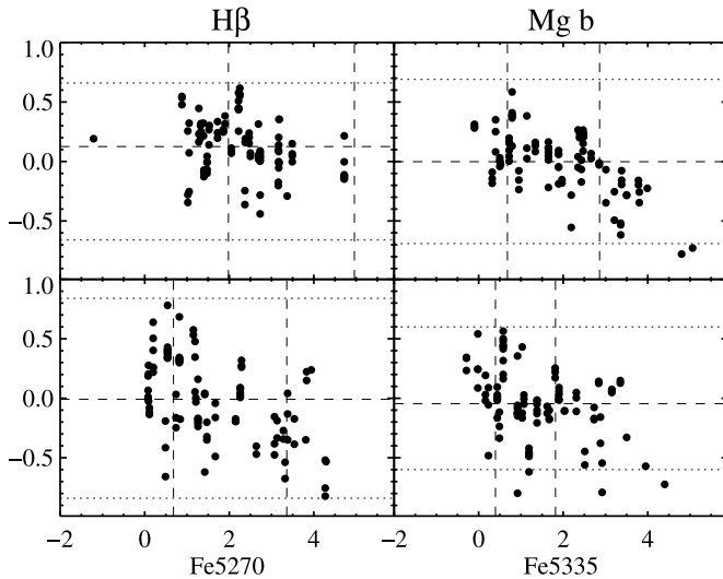
FIG. 2.—Comparison of Lick indices measured with DIS compared to the published equivalent widths in Worthey et al. (1994). Dashed horizontal lines show the mean offsets, while the dotted horizontal lines show the average Worthey et al. \pm 3\sigma uncertainties. Dashed vertical lines show the range of the line indices measured in our galaxy sample. Corresponding means and scatters are given in Table 3.
