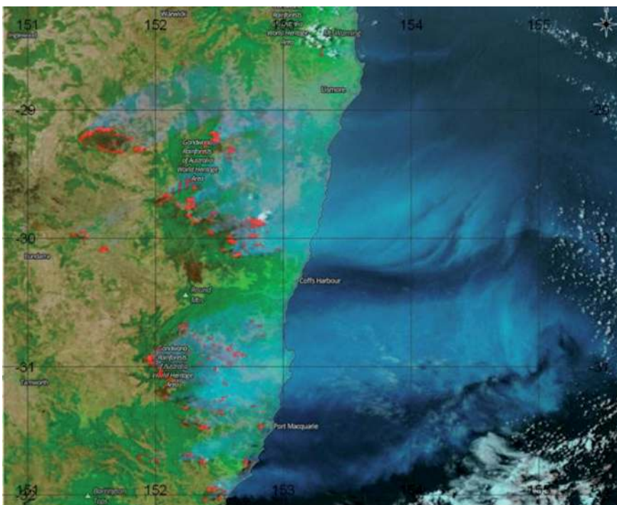
Figure 10. Satellite image of Australia's east coast from 9 November 2019. VIIRS - Suomi NPP sensor (combination: M11-M12-M1).
