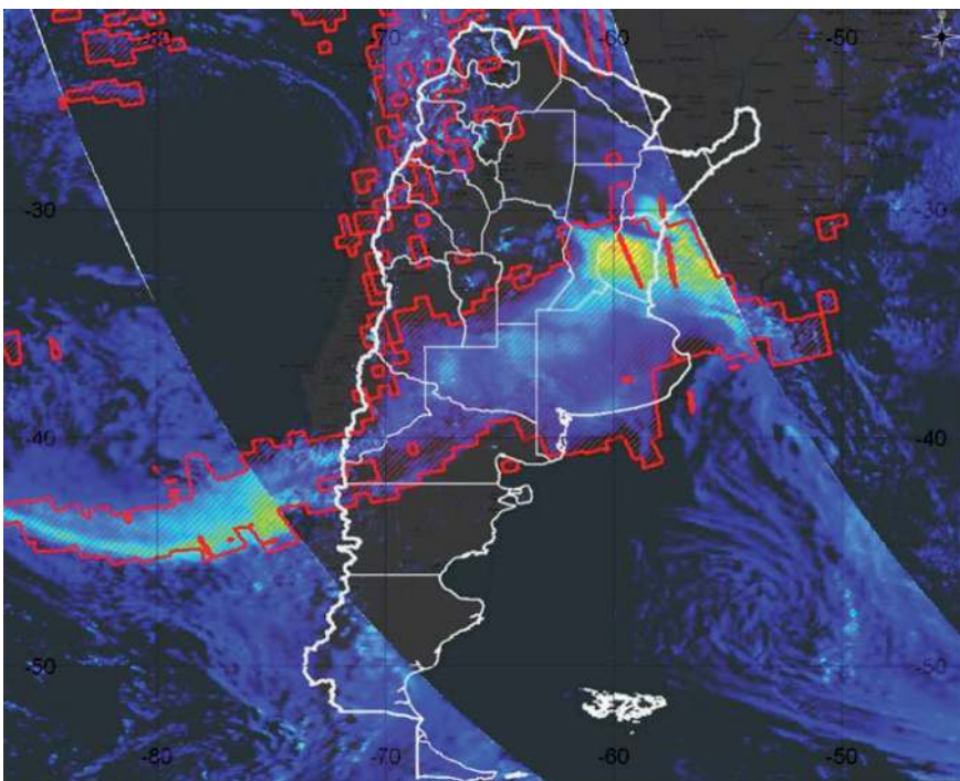
Figure 14. Comparison of the Aerosol Index (AI) coverages, calculated with the TROPOMI sensor (in color palette) and the OMPMS sensor (polygon in red), for 14 November 2019.
