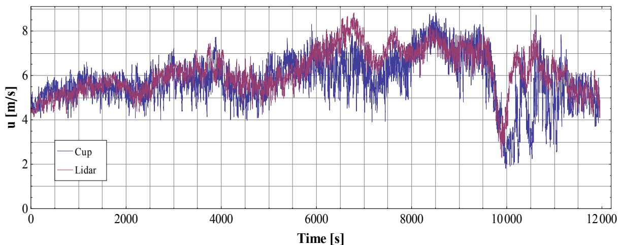
Figure 7: Spinner-lidar measured wind speeds near hub height (purple curve) inter-compared with cup anemometer measured wind speeds in the met mast (blue curve), during a 3-Hour data sampling period on the night of April 30, 2009. Data rate for lidar = 50Hz; Data rate for mast = 10Hz.
