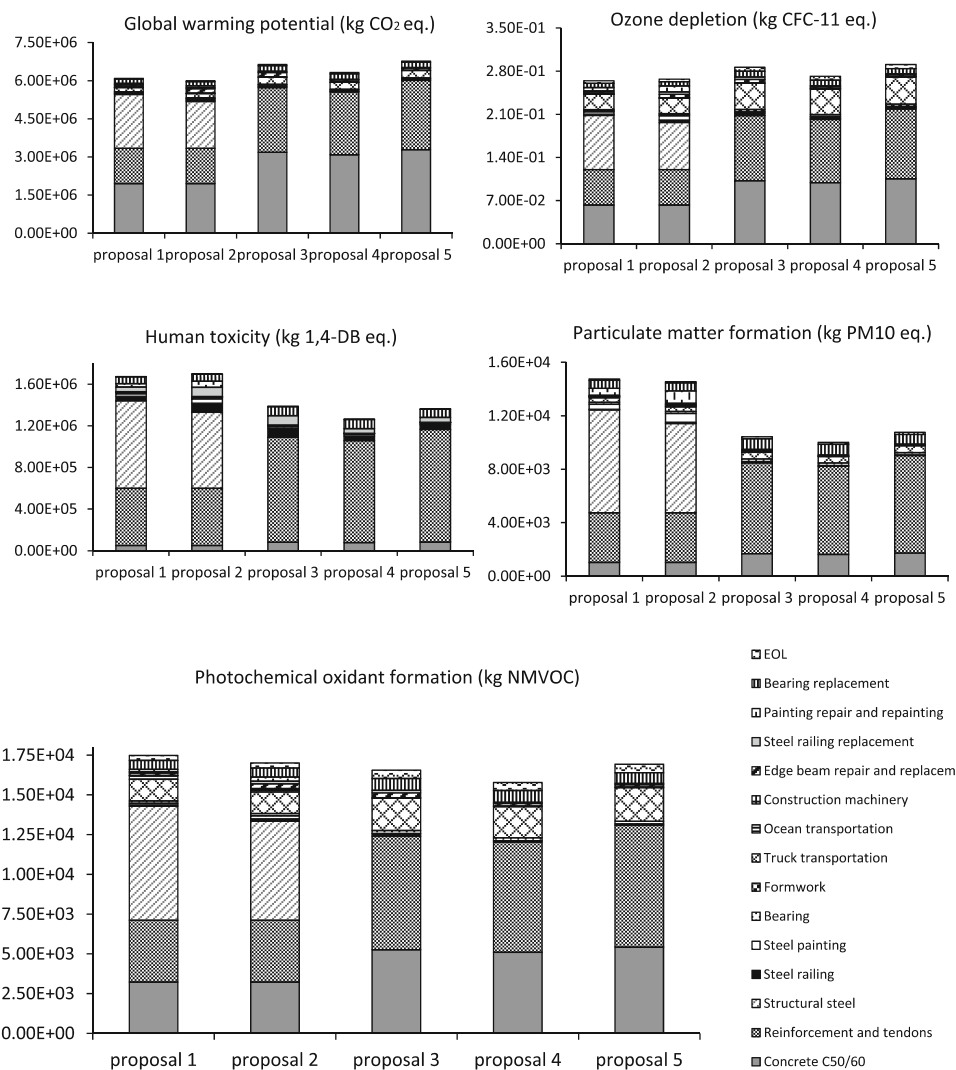
Fig. 6 Environmental impacts of structural components and life cycle measures of the five proposed bridges (unit: kilograms)
