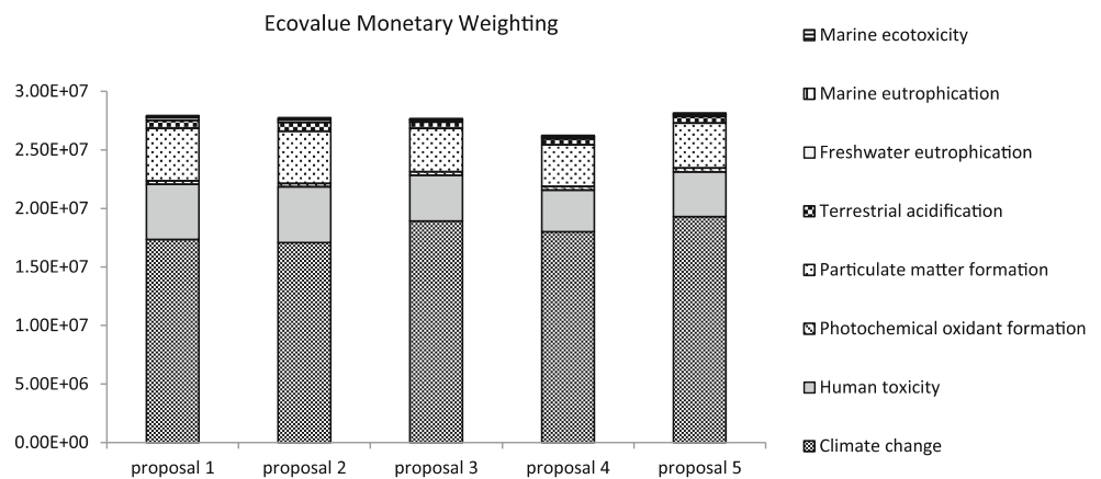
Fig. 10 Environmental costs of the five proposed bridges (SEK)
