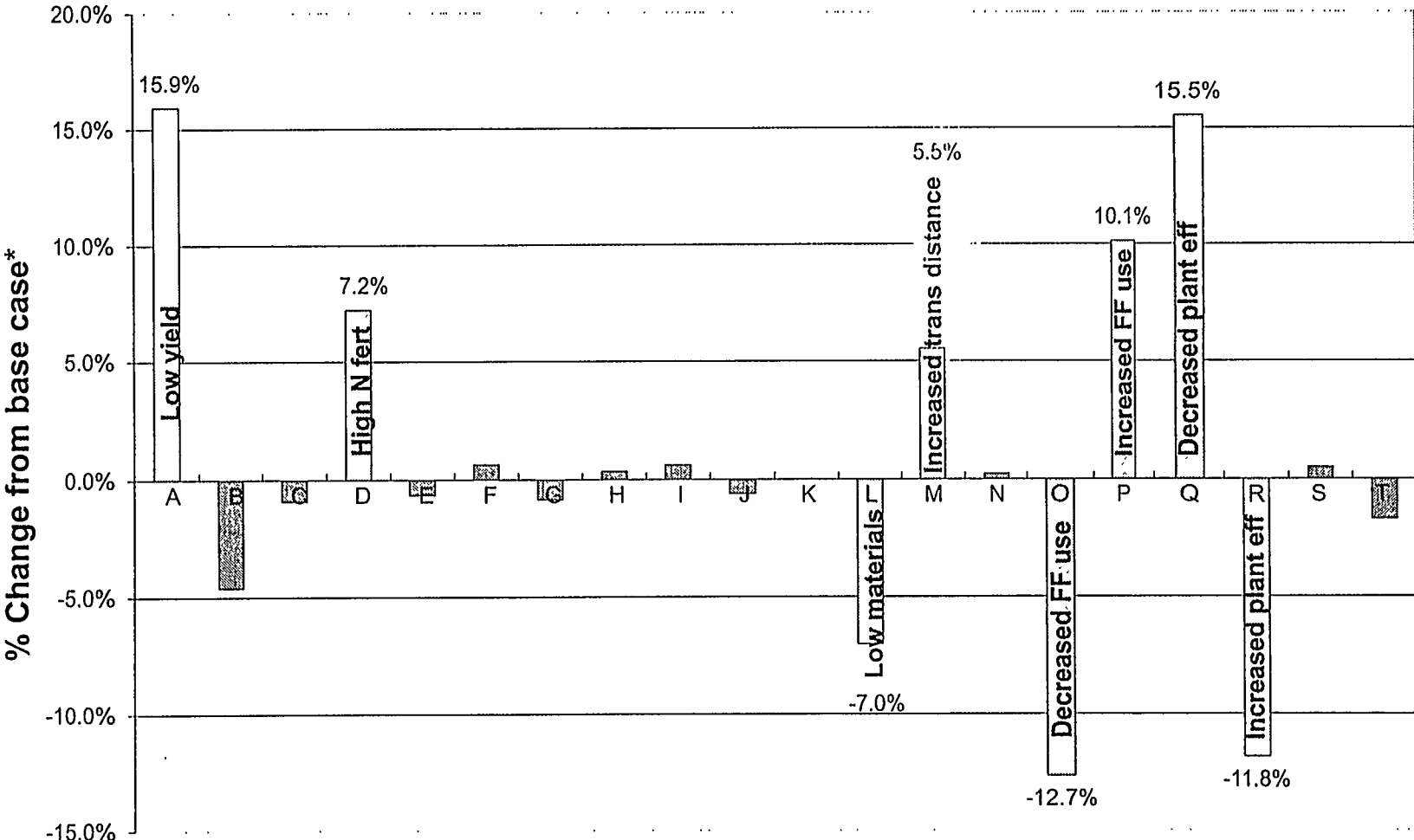
Figure 30: Sensitivity Analysis Results of Net CO 2 Emissions per MWh of Energy Produced
