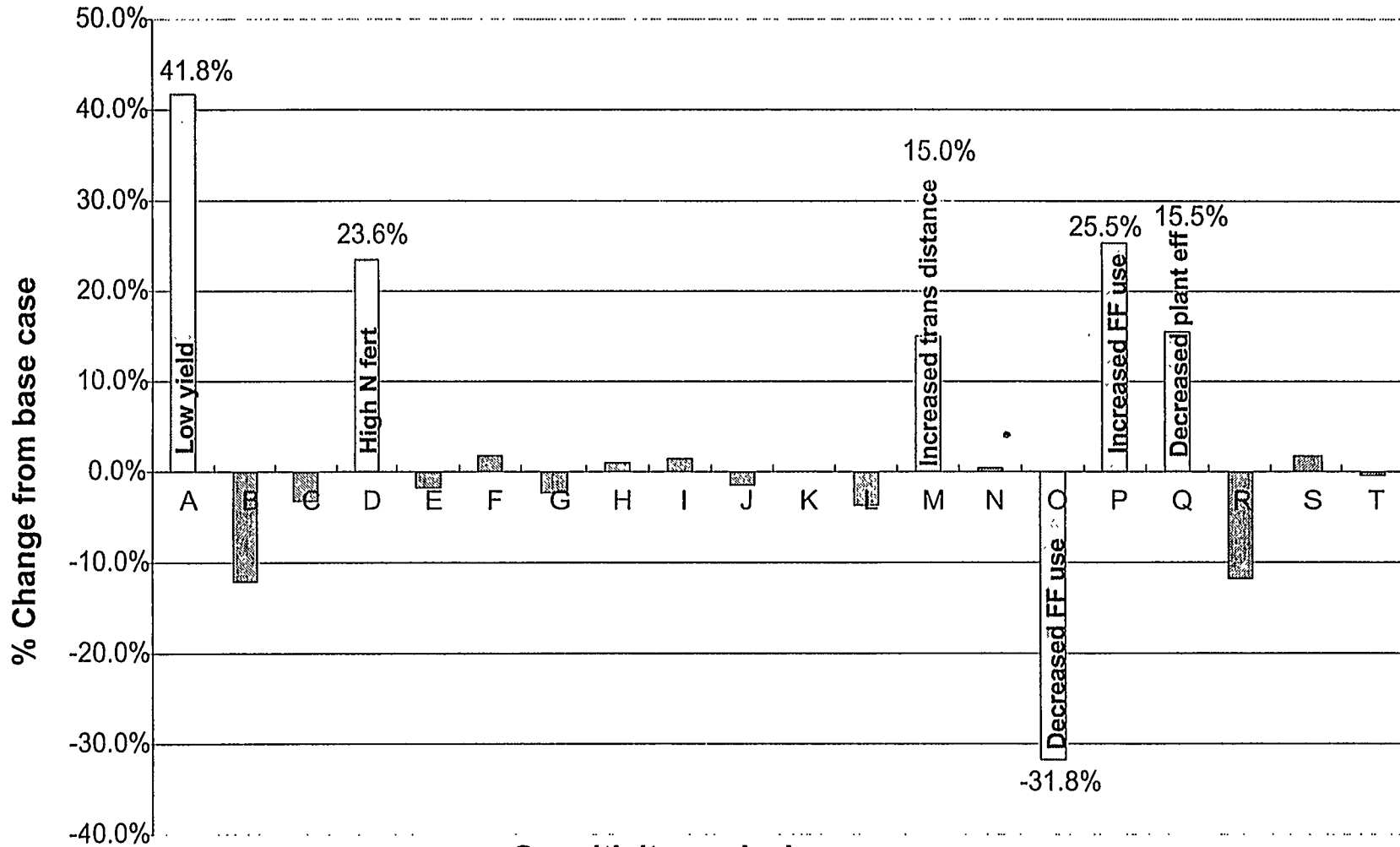
Figure 31: Sensitivity Analysis Results of System Energy Consumption per MWh of Energy Produced
