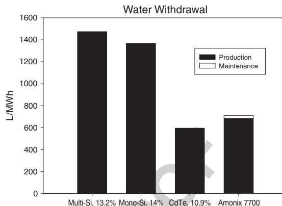
Figure 5. Comparison of water withdrawal across photovoltaic technologies under the environmental conditions of Phoenix, AZ, USA [15].
