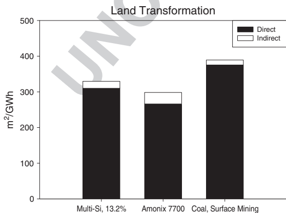
Figure 4. Comparison of land transformation. Photovoltaic technologies are assessed under the environmental conditions of Phoenix, AZ, USA, whereas the coal case refers to surface mining in the Eastern USA (case 1, Table 1 in Ref.[14]).
