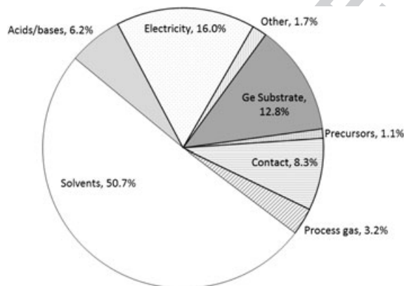
Figure 3. Breakdown of primary energy demand to manufacture III–V solar cells used in Amonix 7700 (total = 14 562 MJ p ).
