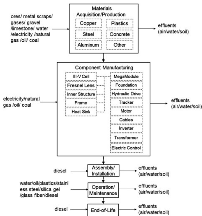
Figure 2. Life cycle flow of Amonix 7700 concentrated photovoltaic.
