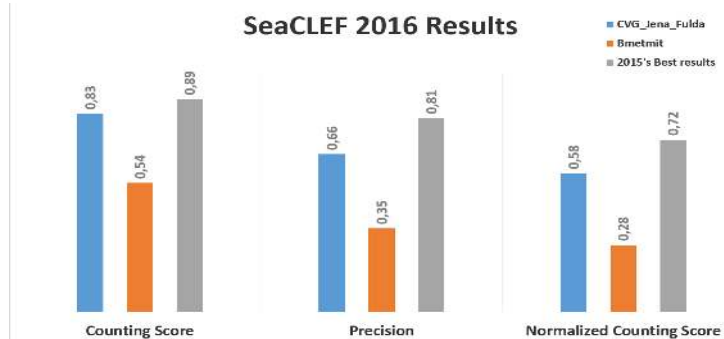
Fig. 3. SeaCLEF 2016 Results.
