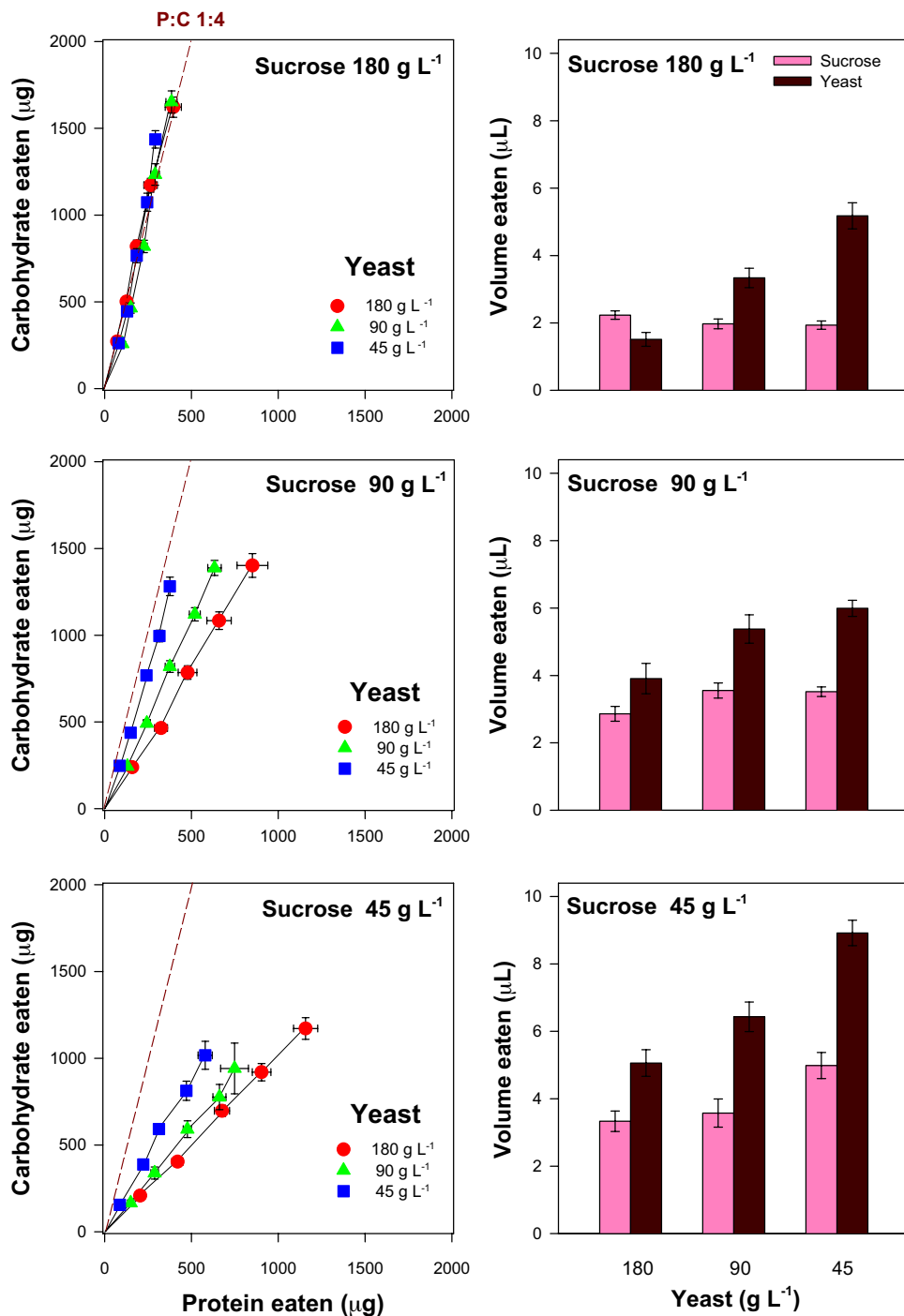
Fig. 3. Mean \pm SEM for macronutrient intake and volume consumed by flies provided with a 5- \mu l glass capillary containing one of three concentrations of yeast (Y) solution and another capillary with one of three sucrose (S) concentrations. (Left) Cumulative protein-carbohydrate intake trajectories at 3-day intervals over 15 days. (Right) This column plots the volume of the solutions imbibed over the first 6 days. In four treatments (S:Y 180:180, 180:90, 180:45, and 90:45), flies converged on a P:C 1:4 trajectory, which maximized lifetime egg production in no-choice experiments (Fig. 1). In the other five choice treatments, the P:C trajectory was more protein-biased because of flies compensating for limiting carbohydrate by feeding from the yeast solution, rather than by increasing intake of dilute sucrose, with associated longevity costs (Fig. 4).
