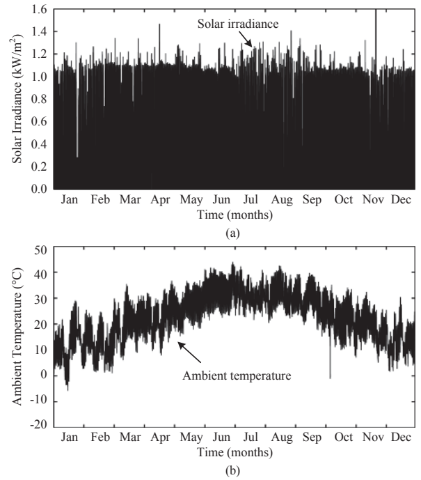
Fig. 3. Yearly mission profiles from the installation site in Arizona with a sampling rate of 5 mins per sample: (a) solar irradiance and (b) ambient temperature.
