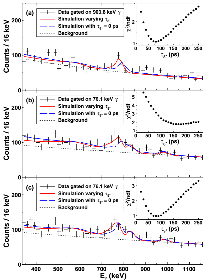
FIG. 4. (color online) Fits to the Doppler-corrected \gamma\gamma coincidence data, with all panels showing the \gamma -rays in the forward ring. In each panel the solid curve is the best fit to the data while the short-dashed line indicates the assumption of the background. The long-dashed curve shows a simulation with a lifetime of 0 ps for comparison. Also shown in each panel is the \chi^2 distribution for that fit. Panel (a) shows the fit to the experimental spectrum gated on the 903.8 keV \gamma -ray from the 10^+ state along with simulations in which the lifetime of the 8^+ state is varied. \chi^2 analysis yields a lifetime of \tau_{8^+} = 80(28) ps. Panel (b) shows the experimental data gated on the 76.1 keV \gamma -ray from the 9^+ state but attempts to fit this data with simulations which do not account for the 9^+ lifetime. These simulations fail to reproduce the experimental lineshape and result in a poor \chi^2 distribution. Panel (c) shows the same data, but the simulations include feeding from the 9^+ state (with \tau_{8^+} = 80 ps fixed), as well as allowing for coincidence from above with the 827.7 keV and 980.7 keV \gamma -rays which populate the 9^+ state. This fit reproduces the lineshape of the 8^+ state, and \chi^2 analysis yields a lifetime for the 9^+ state of \tau_{9^+} = 85(30) ps.
