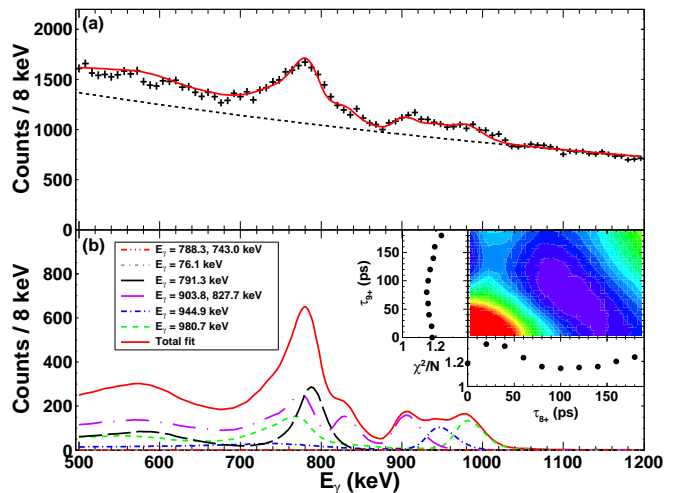
FIG. 6. (color online) (a) The fit to the Doppler-corrected \gamma -ray singles spectrum from the forward detector ring. The fit pictured was generated assuming the lifetimes \tau_{8^+} = 100 ps and \tau_{9^+} = 80 ps. The background was assumed to be exponential in shape and is indicated by the dashed line. (b) The individual components that went into the fit in (a). In contrast to Fig. 3, each component's feeding into the 8^+ state is included in the simulations, with the exception of the 944.9 keV \gamma -ray which does not feed the 8^+ state. Shown in the inset is the \chi^2 surface generated by varying the lifetimes of the 8^+ and 9^+ states, with the projections of the minimum value for each gridline shown along each axis. To provide a sense of scale, the red area in the lower left of the \chi^2 distribution corresponds to a value of \chi^2/N \approx 2 , while the minimum value is approximately \chi^2/N \approx 1.15 . Although the 1\sigma uncertainty limits lie outside the search area, the minimum can be clearly seen at \tau_{8^+} \approx 100 ps and \tau_{9^+} \approx 80 ps, in agreement with the results from the \gamma\gamma coincidence fits.
